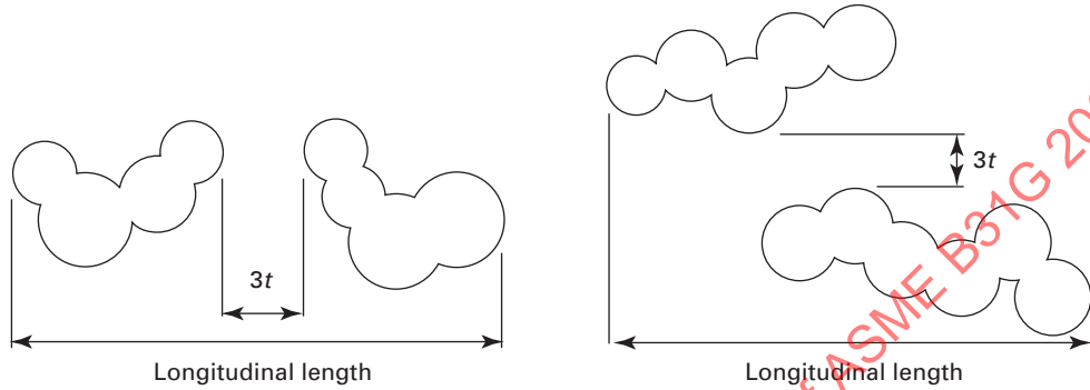
Fig. 1.12-1 Corrosion Pit Interaction Distances
