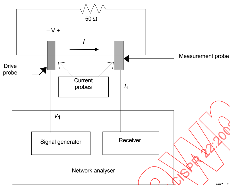
Figure C.4 – Calibration fixture
