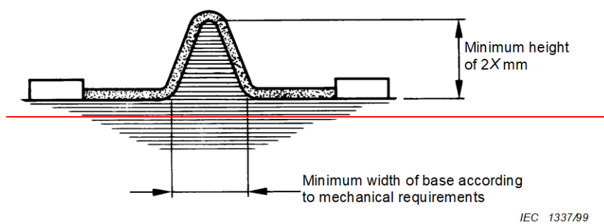
Figure A.1 — Measurement of ribs
