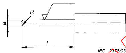
Figure 35 – Gauge dimensions
