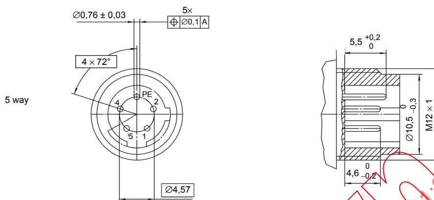
Figure 27 – Pin front view 5 way with C-coding
