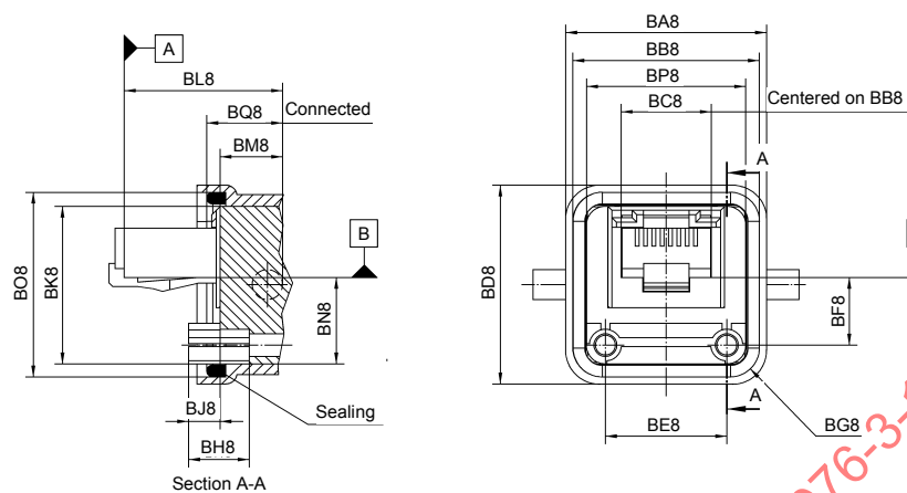
Figure 14 – Variant 07, free connector
