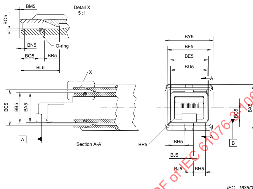
Figure 8 – Variant 04, free connector
