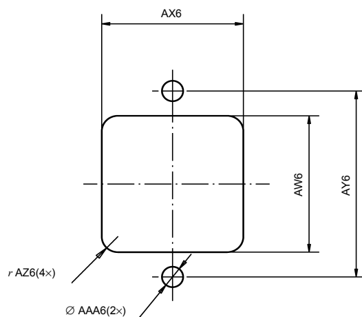
Figure 26 – Variant 05 mounting drawing
