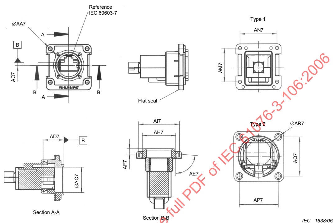
Figure 11 – Variant 06, fixed connector
