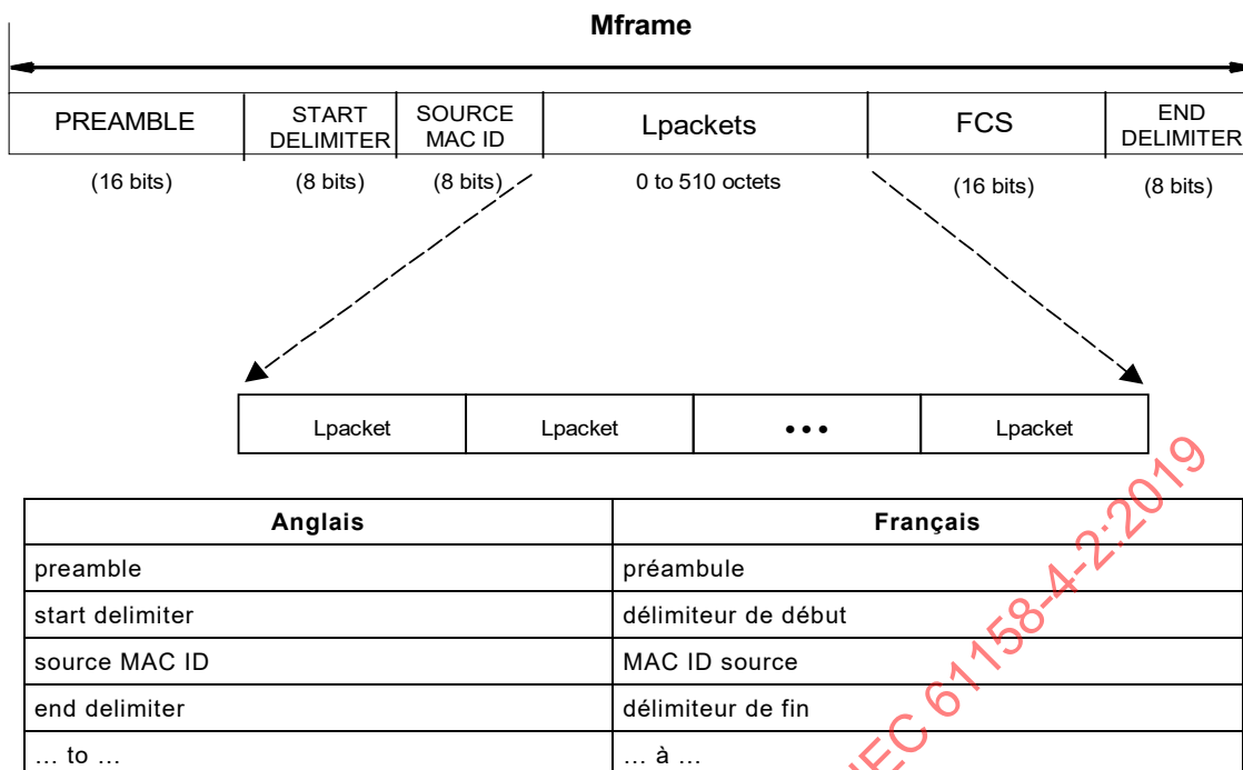
Figure 10 – Format de DLPDU
