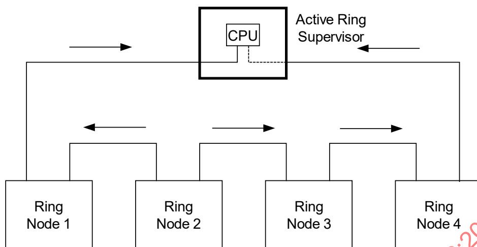
Figure 29 – Normal operation of a DLR network
