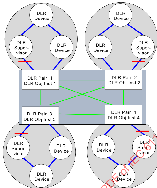
Figure 27 – Devices with Multiple DLR Ring Pairs
