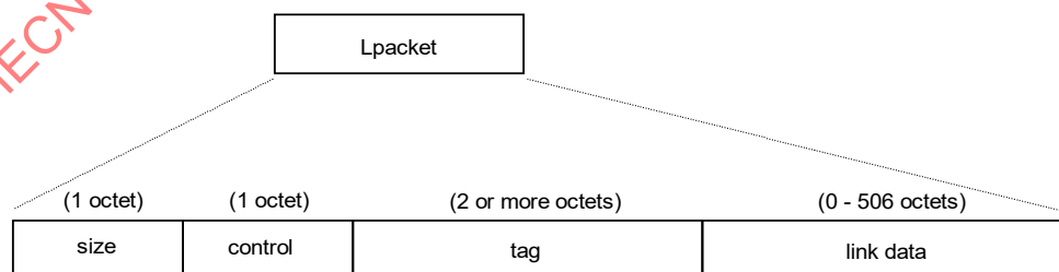
Figure 12 – Lpacket format
