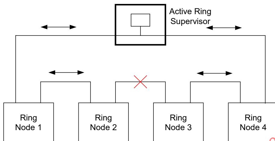
Figure 32 – Network reconfiguration after link failure
