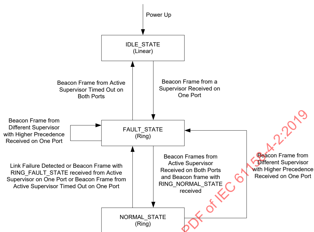
Figure 39 – State transition diagram for Beacon frame based non-supervisor ring node
