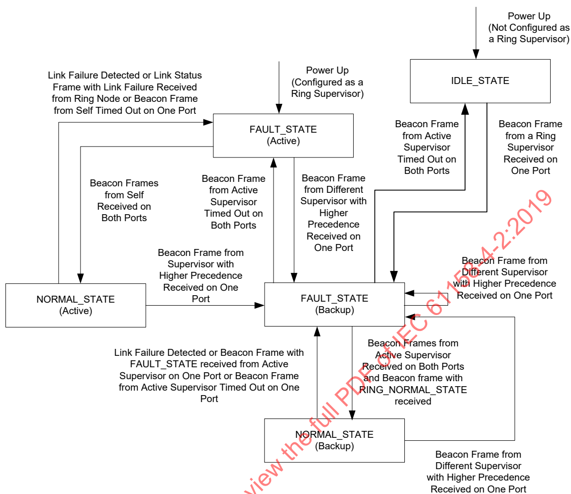
Figure 41 – State transition diagram for ring supervisor
