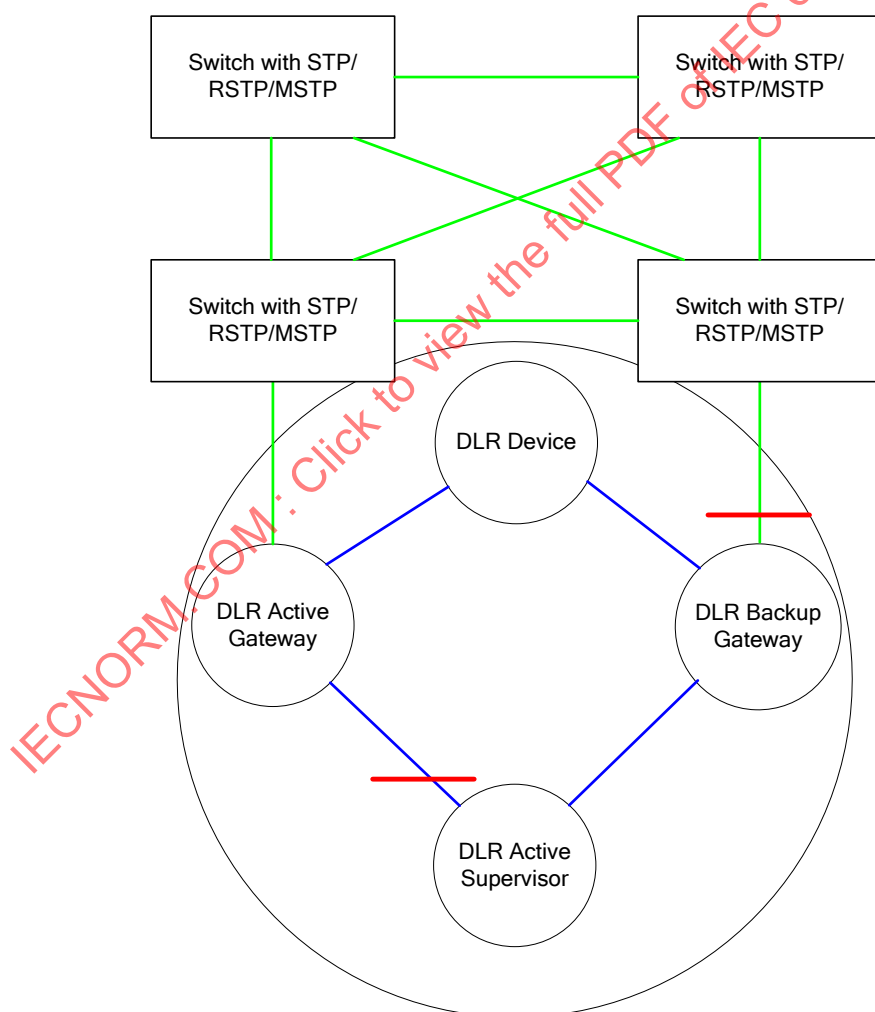
Figure 36 – DLR ring connected to switches through redundant gateways
