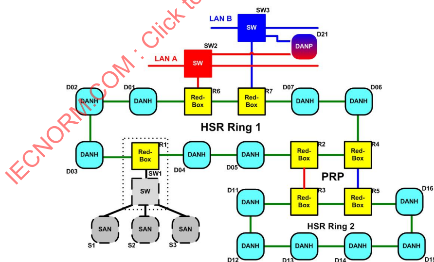
Figure 46 – HSR network
