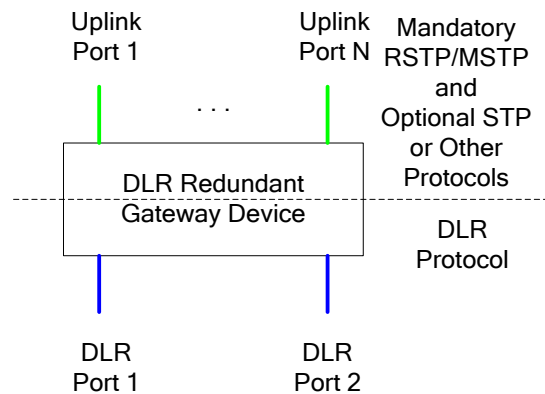
Figure 37 – DLR redundant gateway capable device
