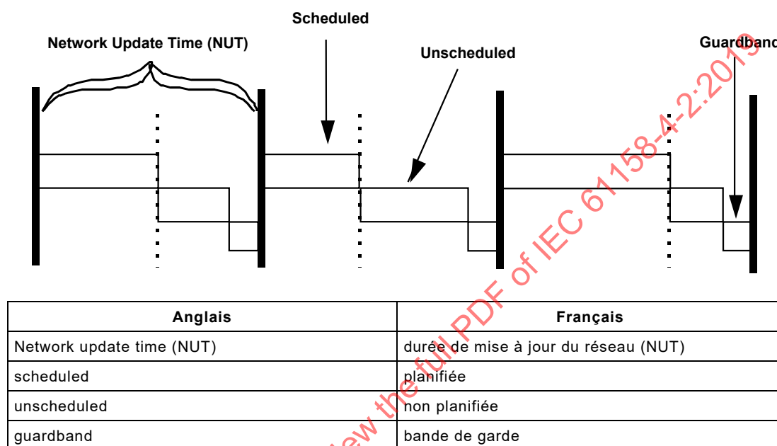
Figure 7 – Structure de la NUT
