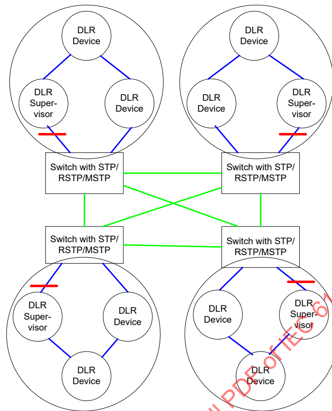
Figure 28 – DLR rings connected to switches
