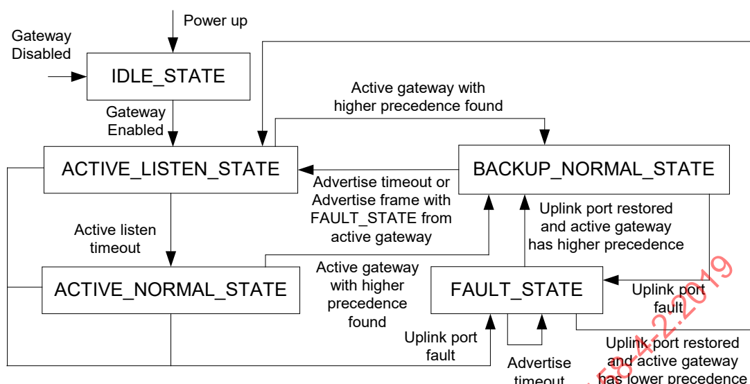
Figure 42 – State transition diagram for redundant gateway
