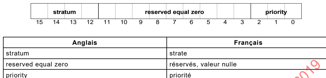
Figure 15 – Paramètre goodness de TimeDist_Lpacket
