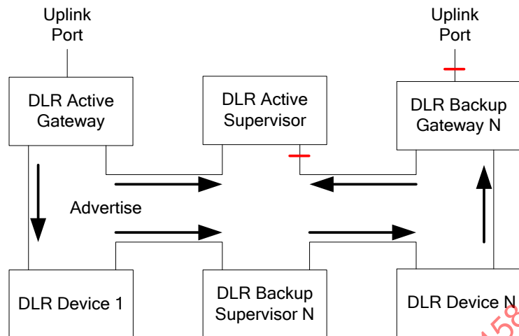
Figure 38 – Advertise frame
