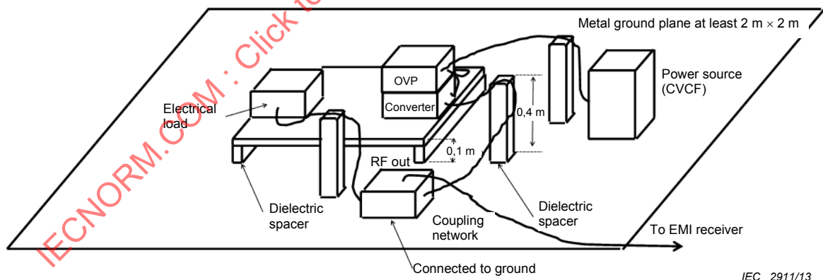
Figure H.4 – Measurement setup of conducted emissions (setup type B)
