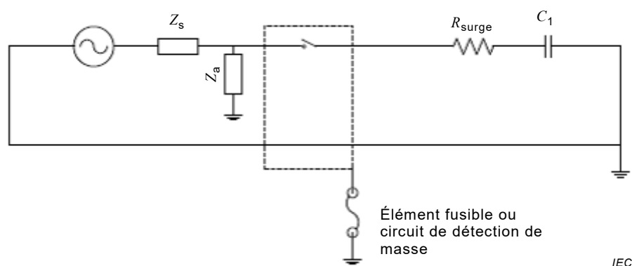
Figure 2b – Circuit monophasé
