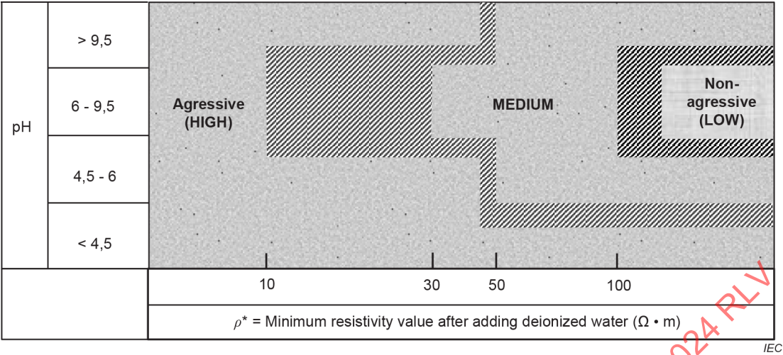
Figure A.1 – Corrosion load (free corrosion without concentration cell)
