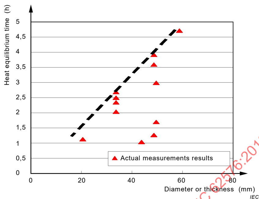
Figure B.2 – Heat equilibrium times of capacitors (from -40\text{ }^{\circ}\text{C} to 25\text{ }^{\circ}\text{C} )
