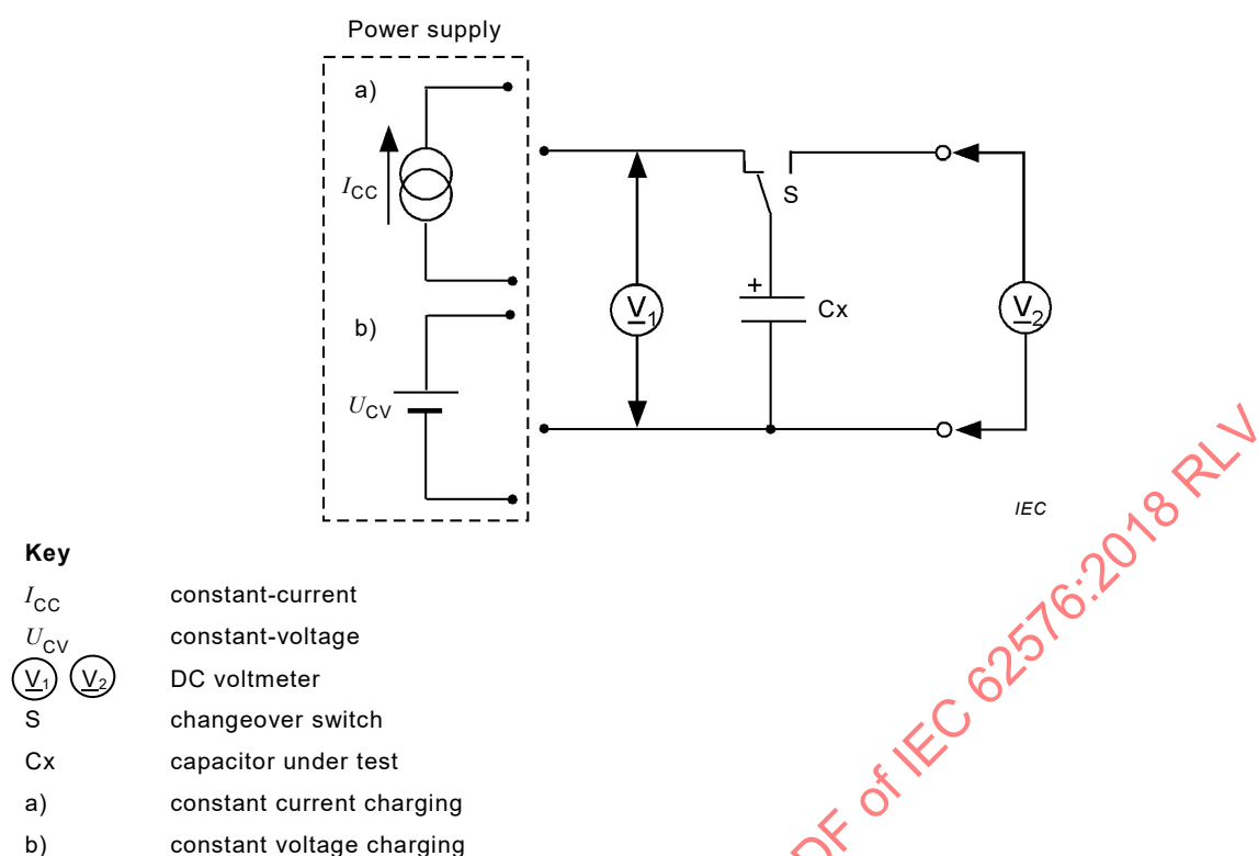
Figure 3 – Basic circuit for measuring the voltage maintenance characteristics
