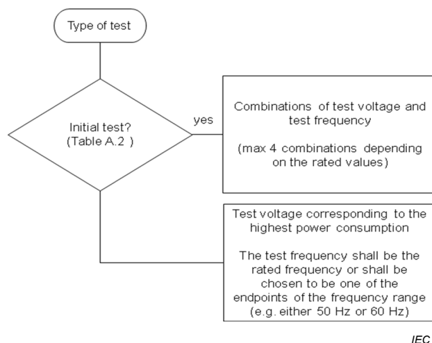
Figure A.3 – Relation of type of tests to test voltage and test frequency
