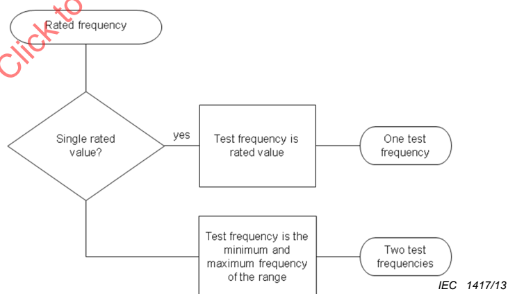
Figure A.2 – Relation of rated frequency to test frequency
