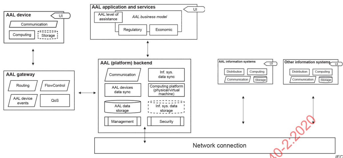
Figure 5 – Illustration of the function layer (functional layer)
