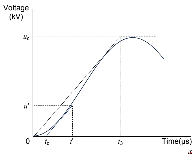
Figure 13 – 2-parameter representation of prospective TRV waveform for interrupting three-phase symmetrical faults
