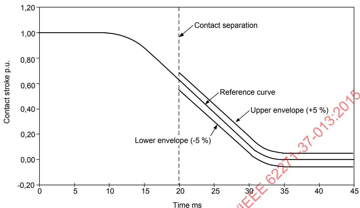
Figure 17 – Reference mechanical travel characteristics (idealised curve) with the prescribed envelopes centered over the reference curve (+5 %, -5 %), contact separation in this example at time t = 20 ms
