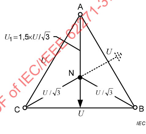
d) Voltage diagram for alternative circuit
