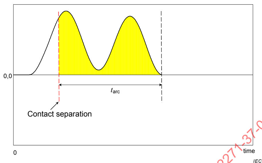
Figure 38 – Example of a valid test for test-duties 6A and 6B
