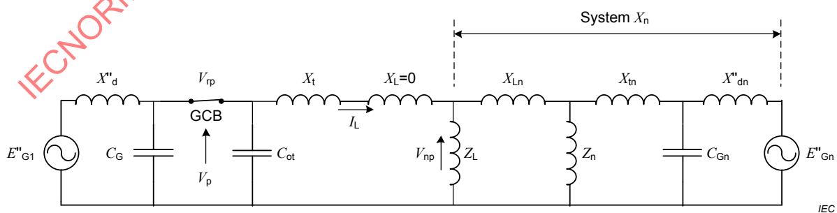
Figure 51 – Single-line diagram of power system
