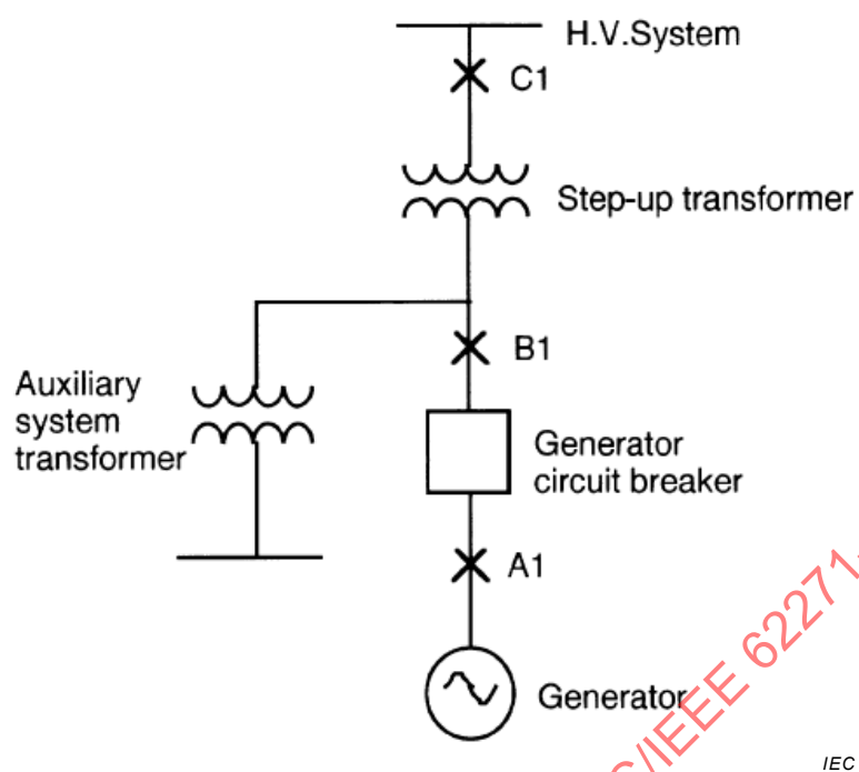
Figure 48 – Single-line diagram of unit generator system
