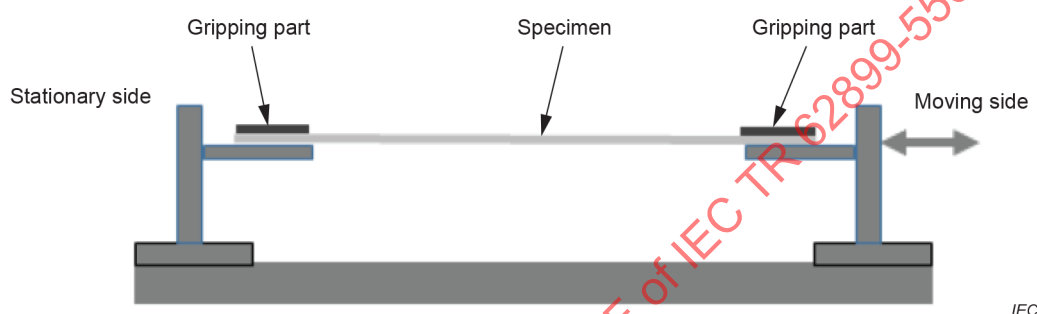
Figure 5 – Stretching apparatus of IEC 62899-502-1
