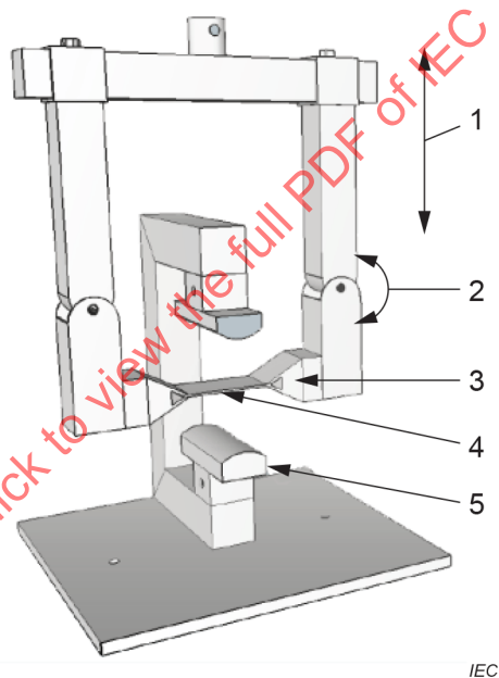
Figure 1 – Bending apparatuses of IEC 62899-201
