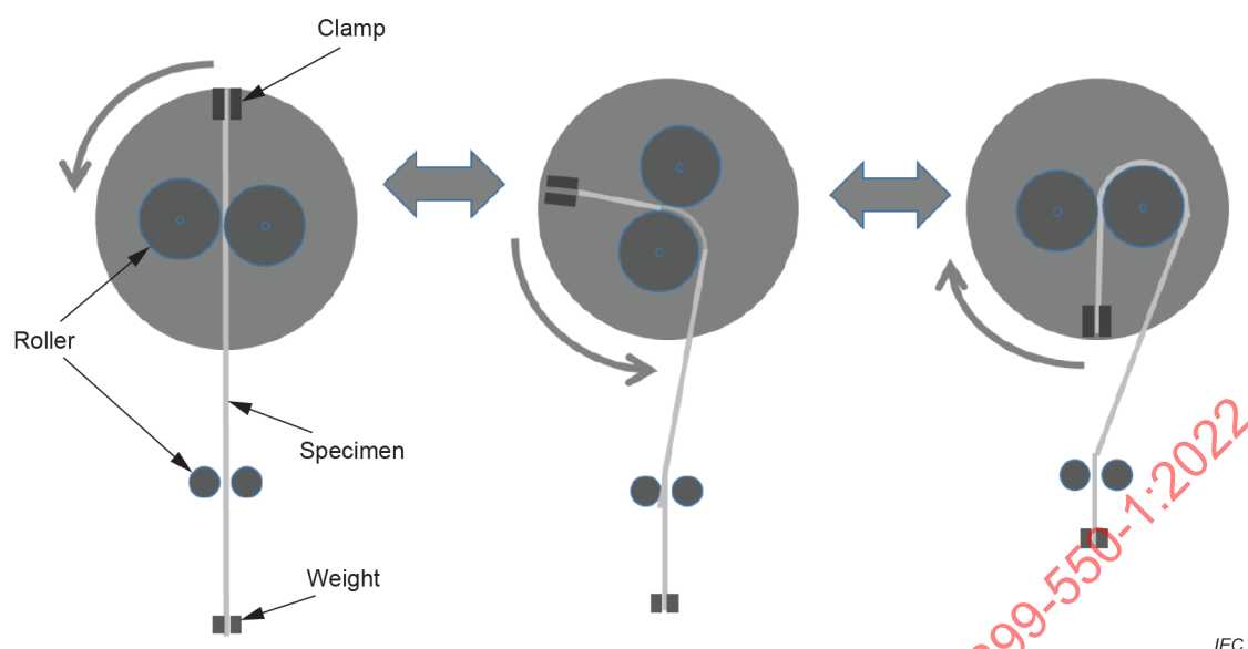
Figure 3 – Bending apparatus of IEC 62899-502-1
