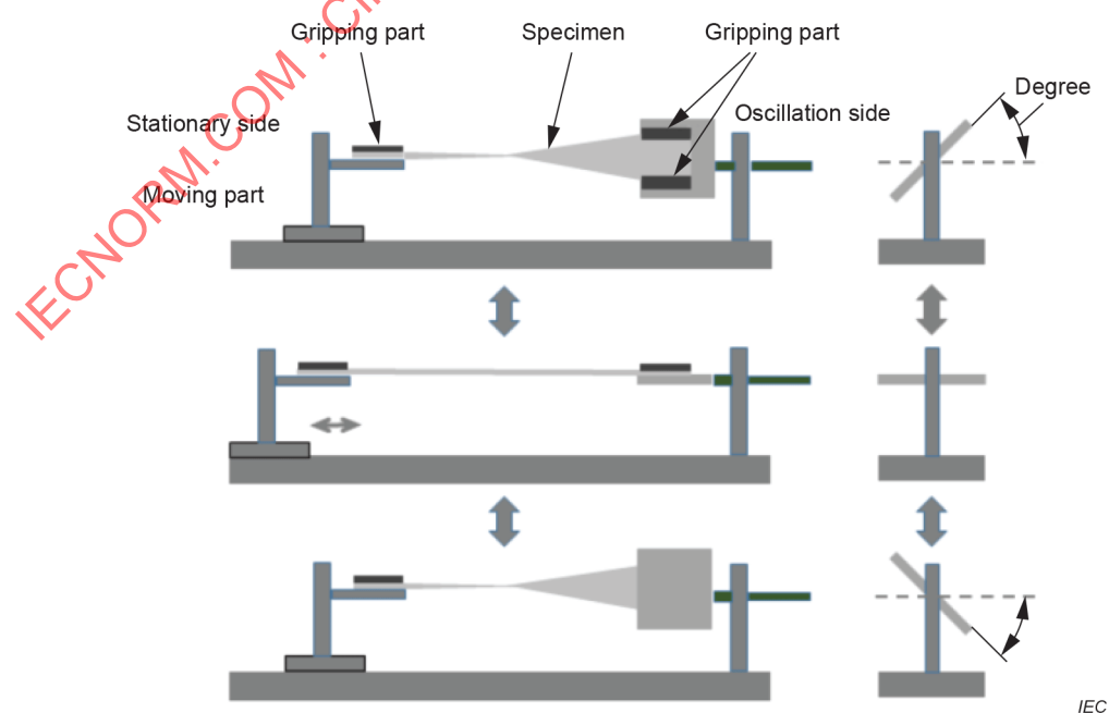
Figure 4 – Torsion apparatus of IEC 62899-502-1
