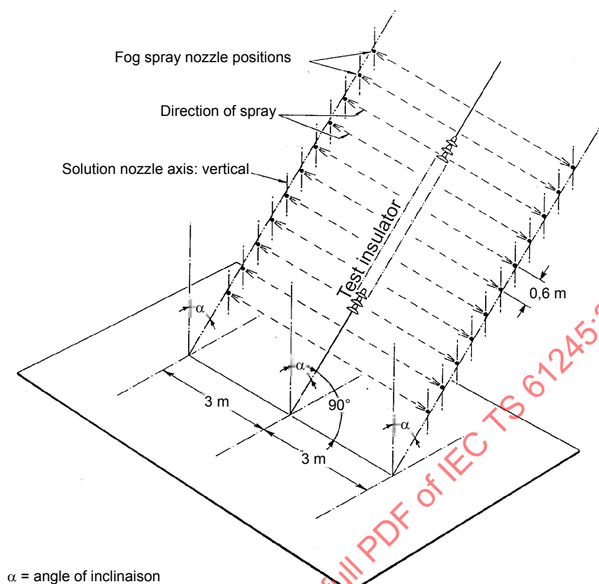
Figure 5 – Test layout for inclined insulators
