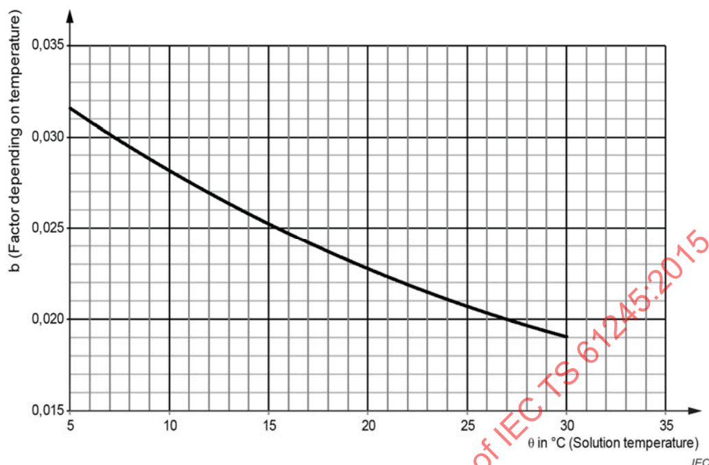
Figure 3 – Value of factor b versus solution temperature θ
