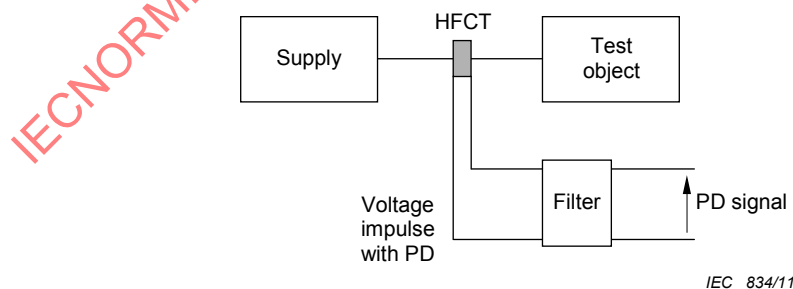
Figure 3 – HFCT between supply and test object with multipole filter
