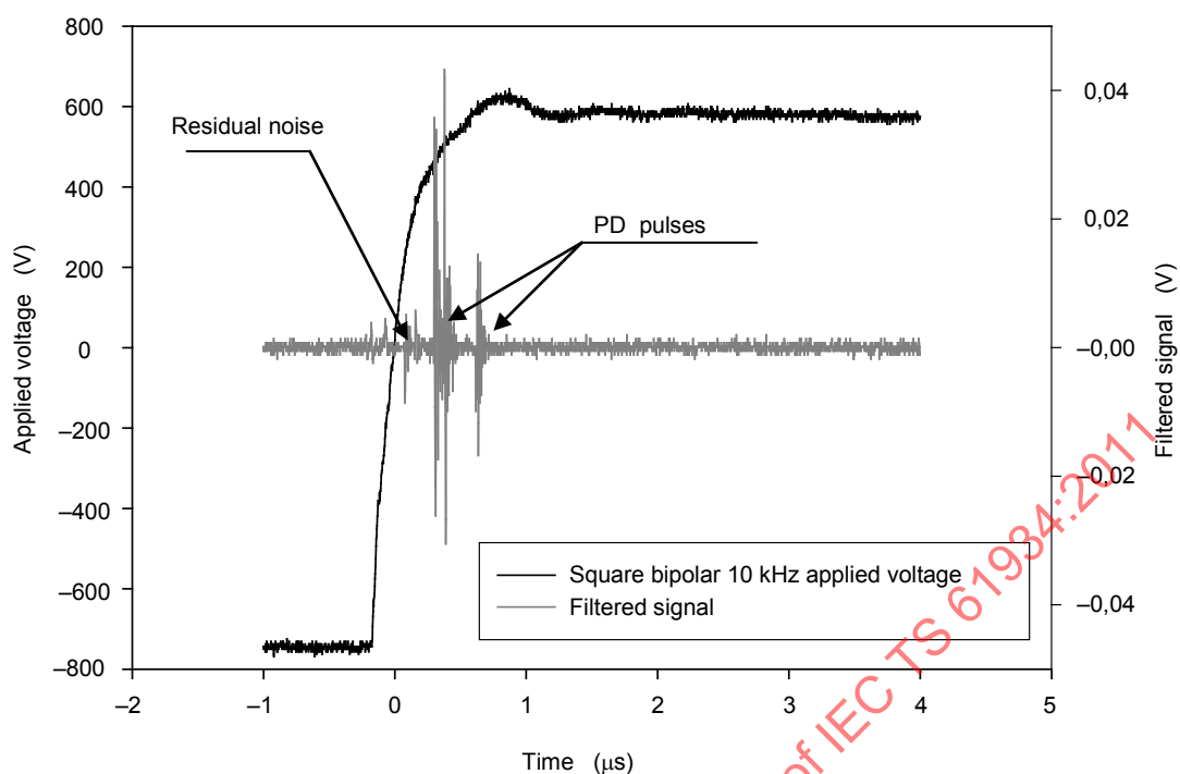
Figure B.2 – Signal detected by an antenna from the record of Figure B.1, using a filtering technique (400 MHz high-pass filter)
