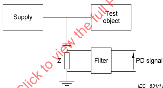
Figure 1 – Coupling capacitor with multipole filter
