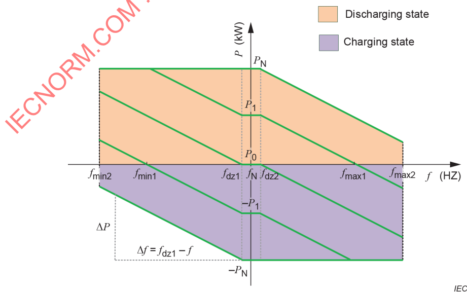
Figure 2 – Typical power-frequency response curve for BESS charging and discharging modes under operating frequency range
