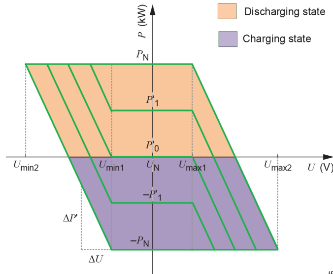
Figure 4 – Typical voltage related active power regulation of BESS
