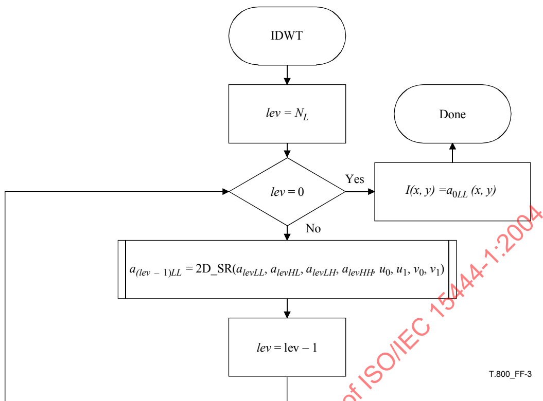
Figure F.3 – The IDWT procedure
