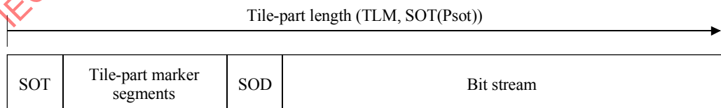
Figure A.16 – Tile-part lengths
