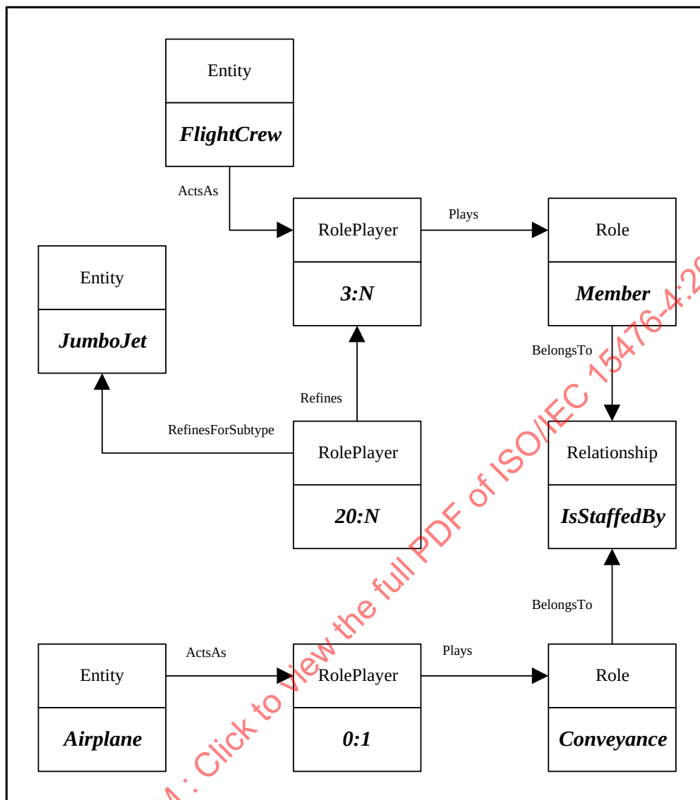
Figure 38 – Instance Diagram showing refinement of Cardinalities.
