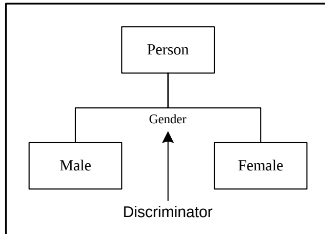
Figure 29 – Subtype Set Discriminator
