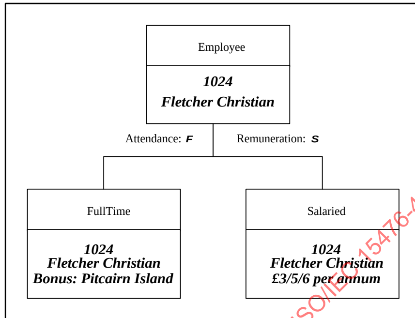
Figure 34 – Instance Diagram showing Orthogonal Subtype Sets
