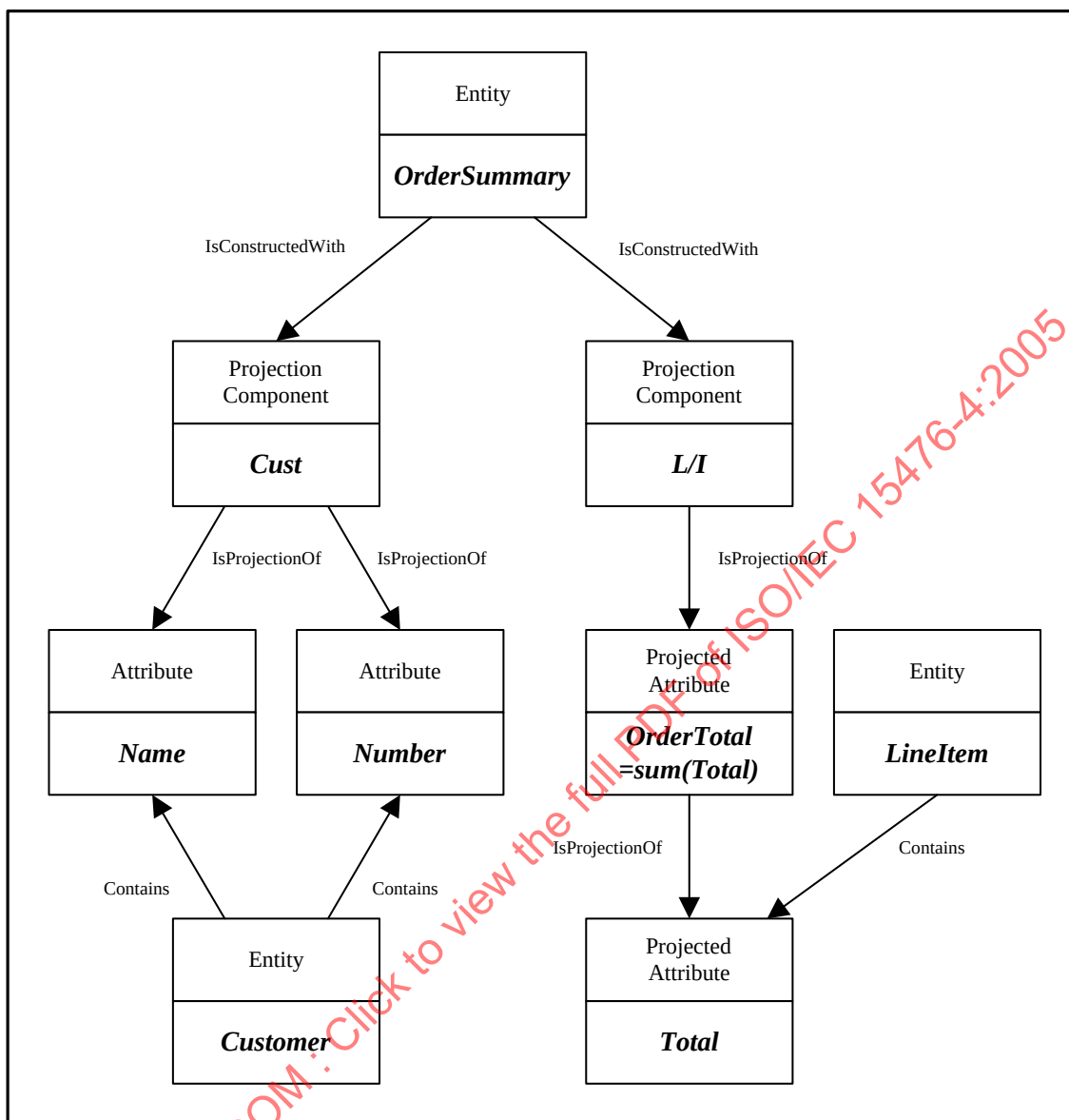
Figure 42 – Instance Diagram showing Complex Projection
