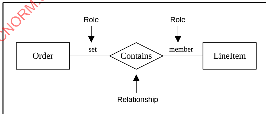
Figure 13 – Roles
