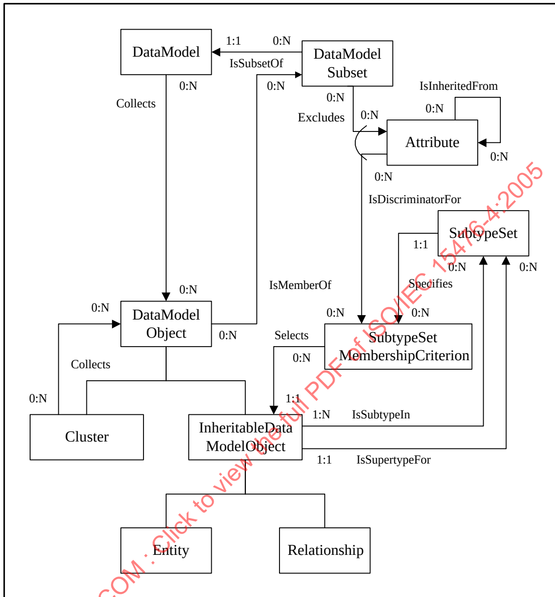
Figure 4 – Partitioning/View mechanisms
