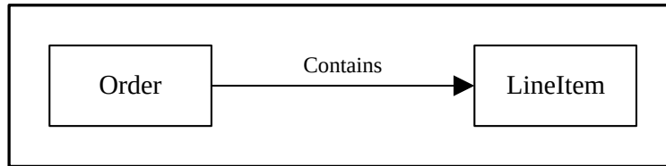
Figure 9 – Binary Relationship
