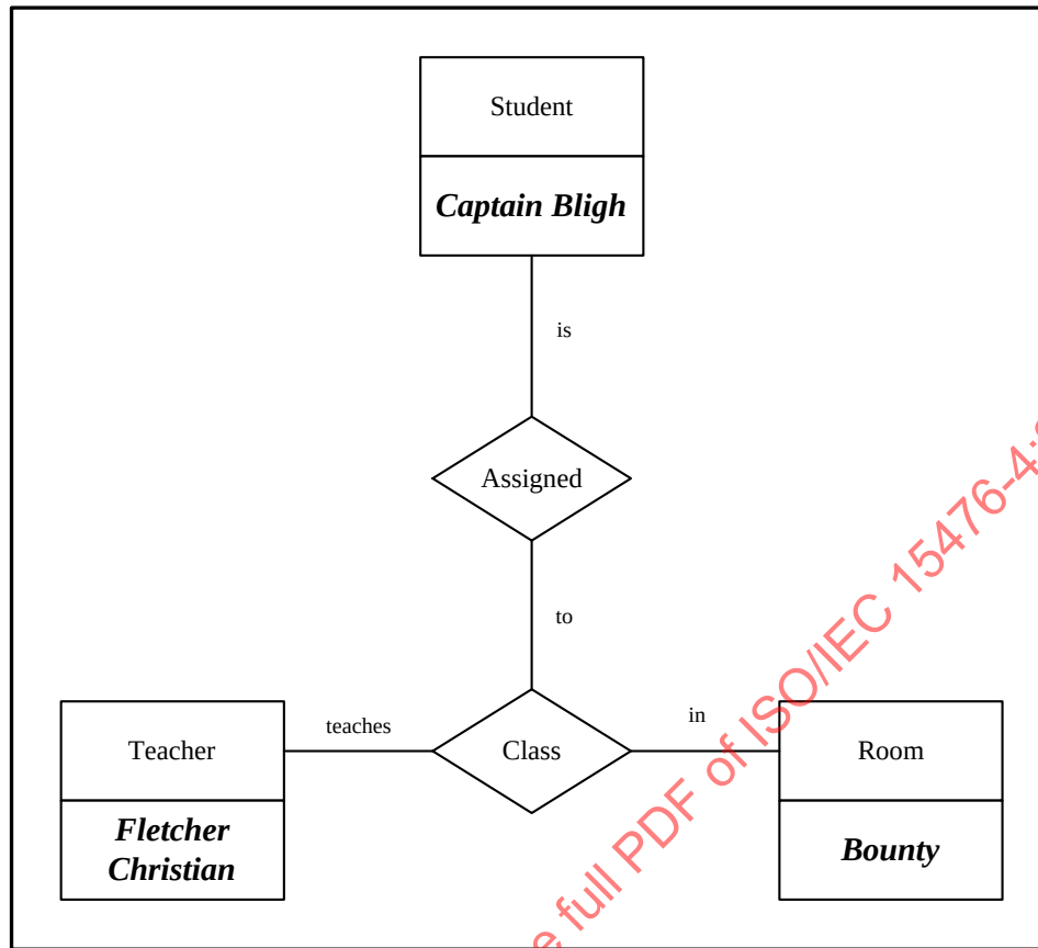
Figure 12 – Instance Diagram showing a Complex Relationship
