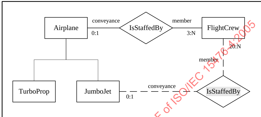
Figure 37 – Refinement of Cardinalities
