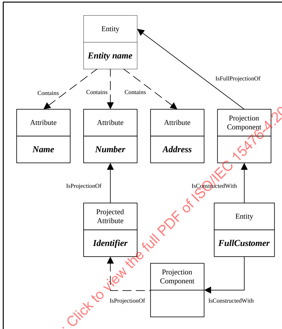
Figure 43 – Instance Diagram showing Attribute Renaming
