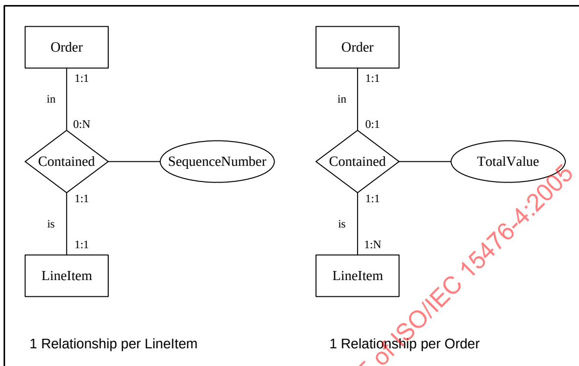
Figure 18 – Inner Cardinalities and Attributed Binary Relationships
