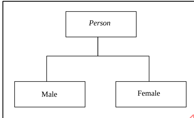
Figure 30 – Abstract Supertype
