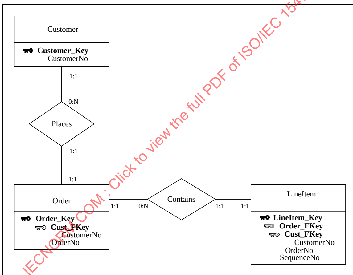
Figure 25 – Foreign Keys
