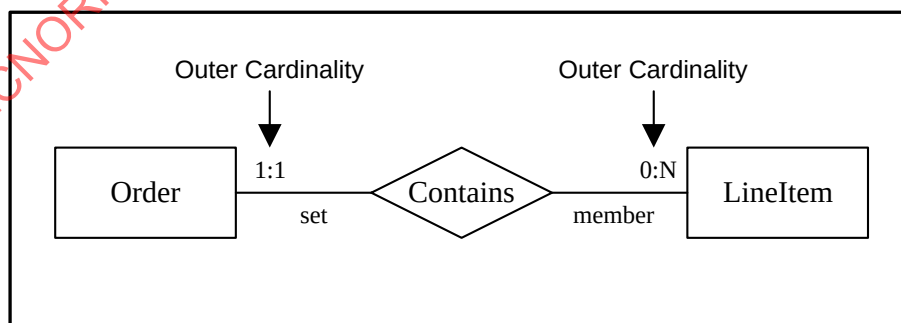
Figure 16 – Outer Cardinalities
