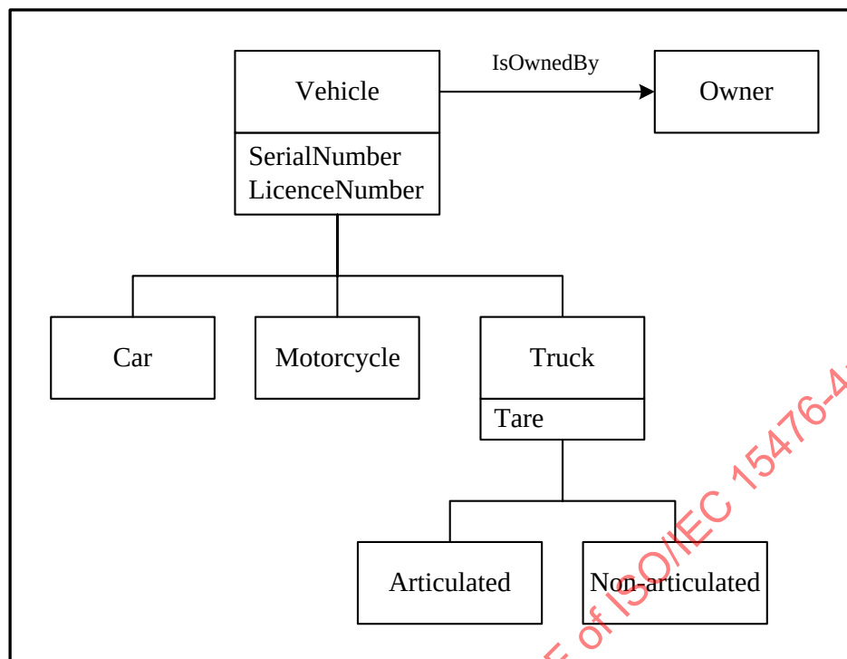
Figure 36 – Inheritance
