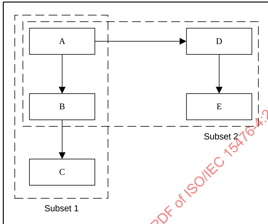
Figure 39 – Subsets
