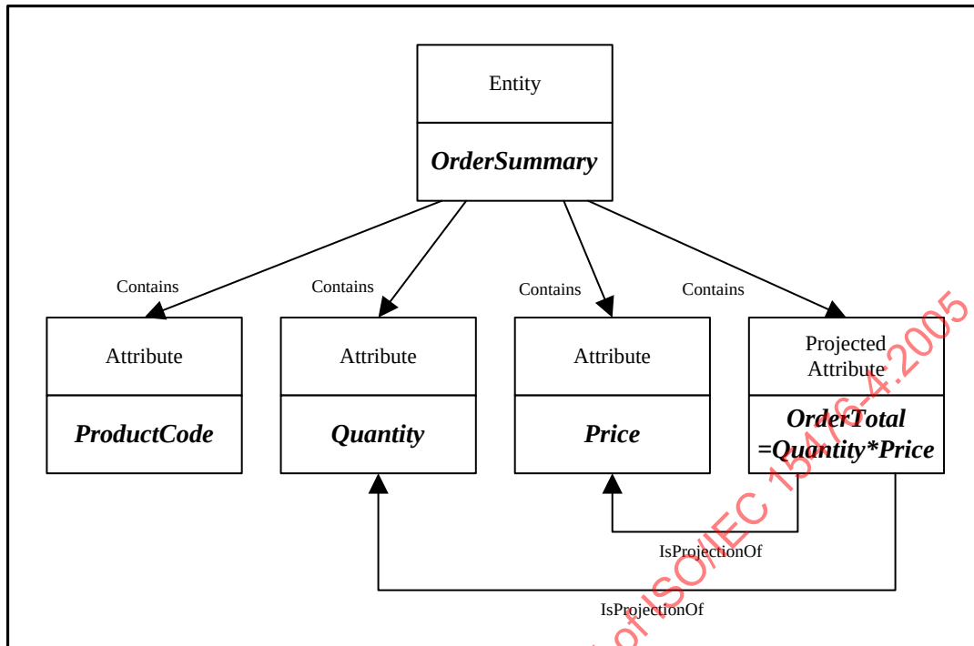
Figure 41 – Instance Diagram showing Simple Projection
