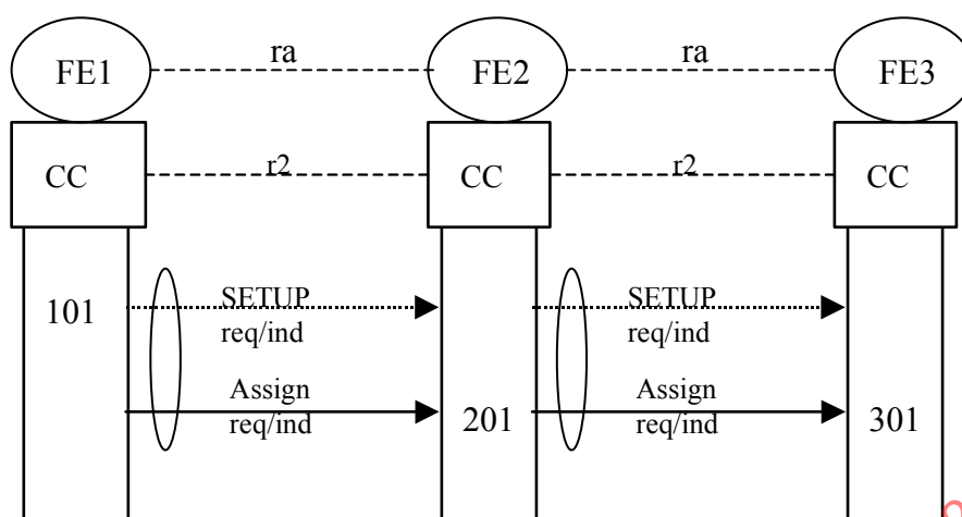
Figure 4 - Information Flow Sequence - Normal Operation of ANF-CIDL, assignment of call identification data for a new call
