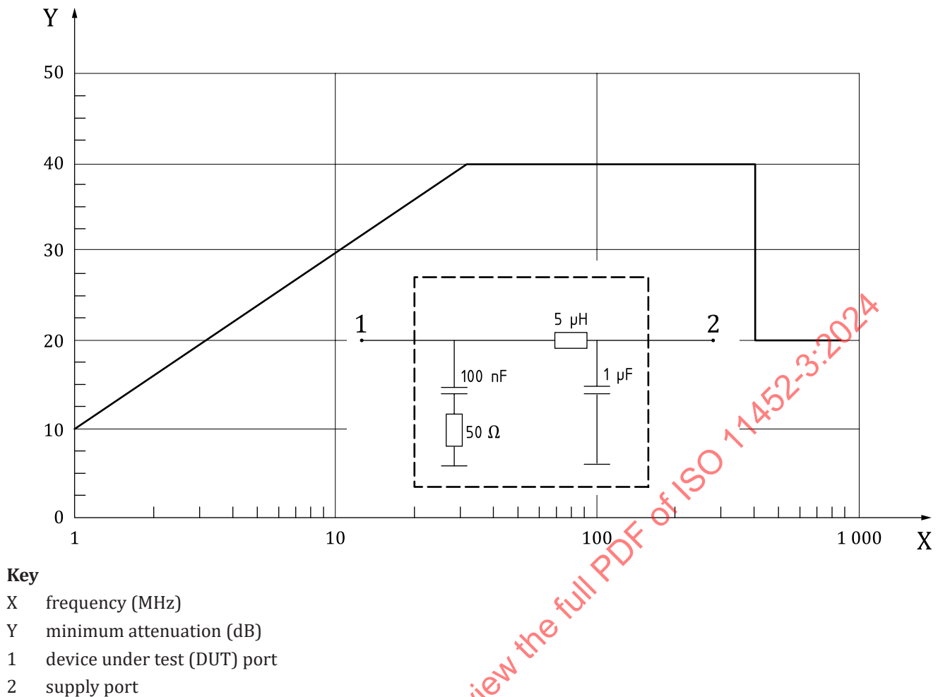
Figure C.1 — Minimum attenuation and frequency response of the low pass filter with schematic circuit diagram (artificial network)
