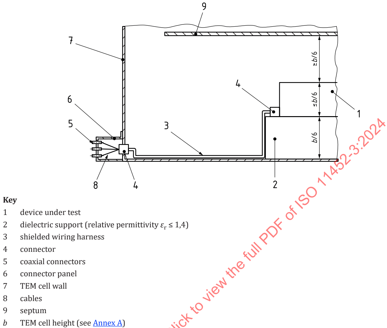
Figure 5 — Example test set-up — Major field coupling to device under test (side view)
