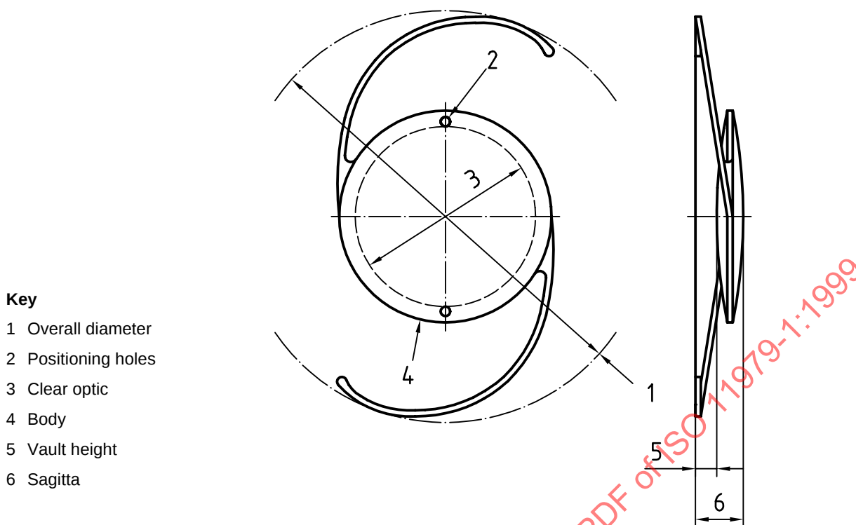
Figure 1 — Overall diameter, vault height, sagitta, clear optic, body and positioning hole
