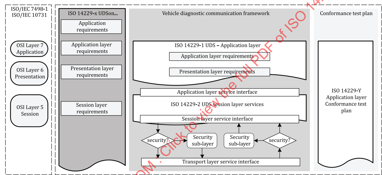
Figure 1 — ISO 14229 series reference according to OSI model
