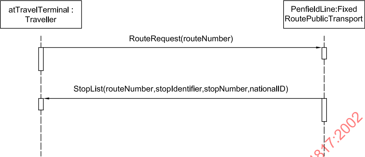
Figure E.5 — Interaction diagram for bus query
