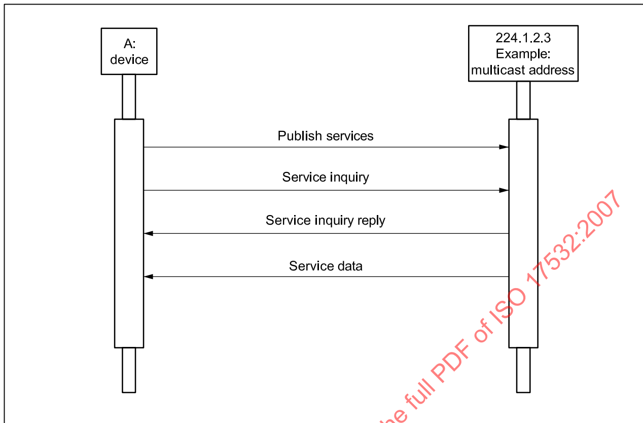
Figure 5 — Boot-up sequence — Type 1
