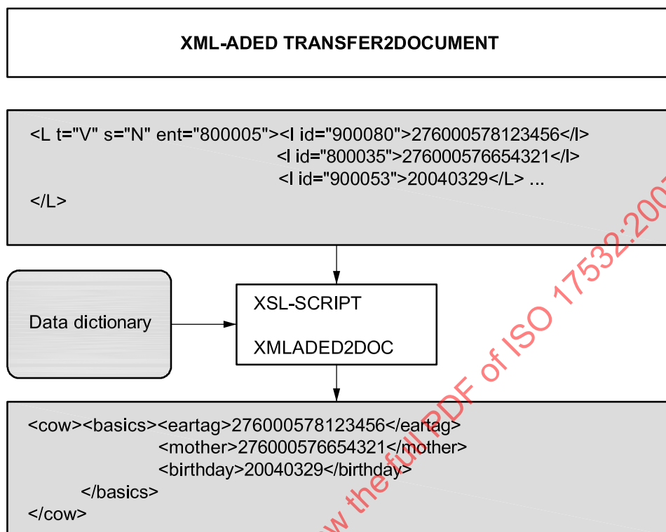
Figure 10 — Transforming XML/ADED into humanly readable XML documents
