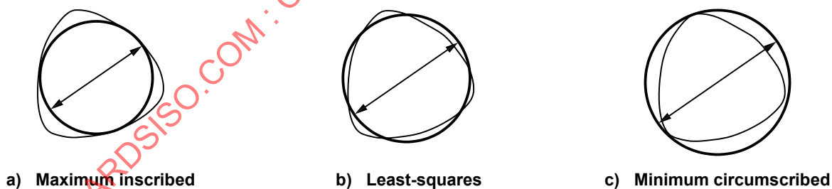
Figure 27 — Independent size characteristic of a nominally circular line with different criteria of association
