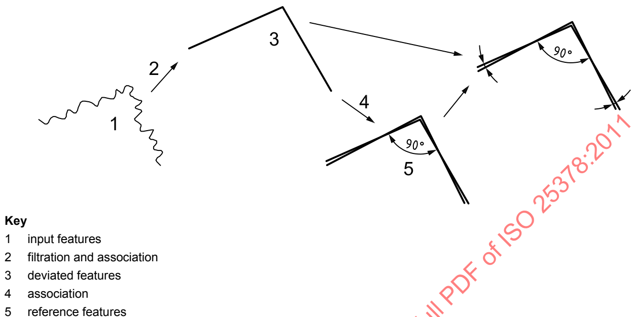
Figure 28 — Independent orientation characteristic
