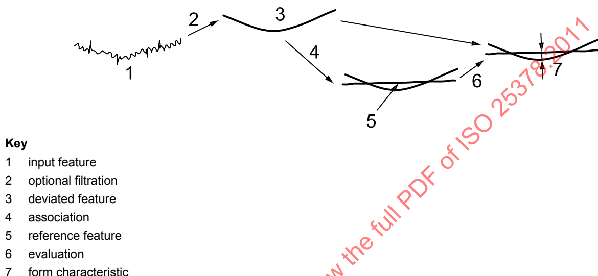
Figure 20 — Independent form characteristic
