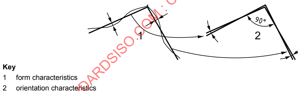
Figure 29 — Independent and complementary form and orientation characteristics of two nominally straight lines
