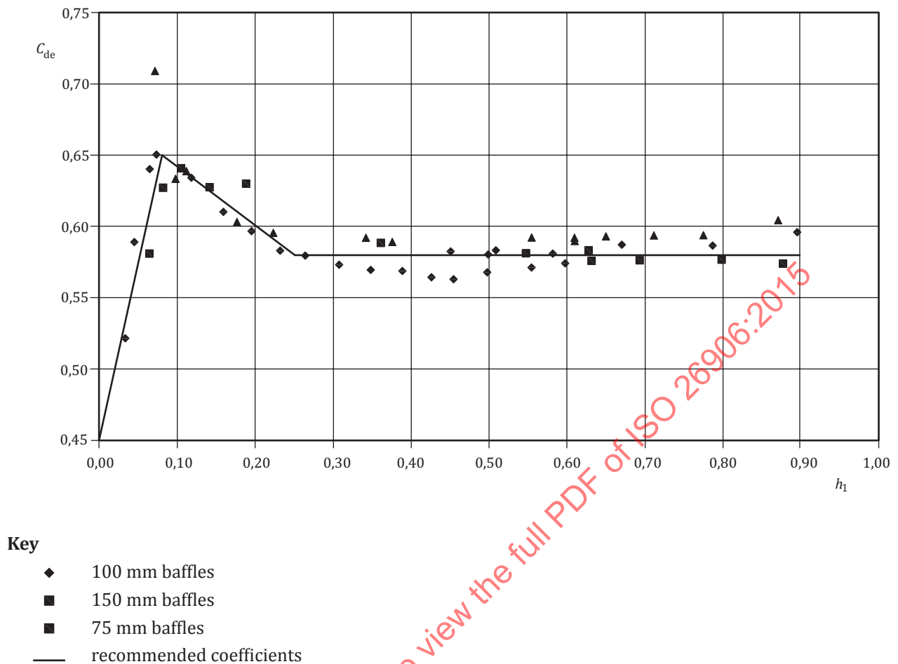
Figure 3 — Coefficient of discharge for super-active Larinier fishpass
