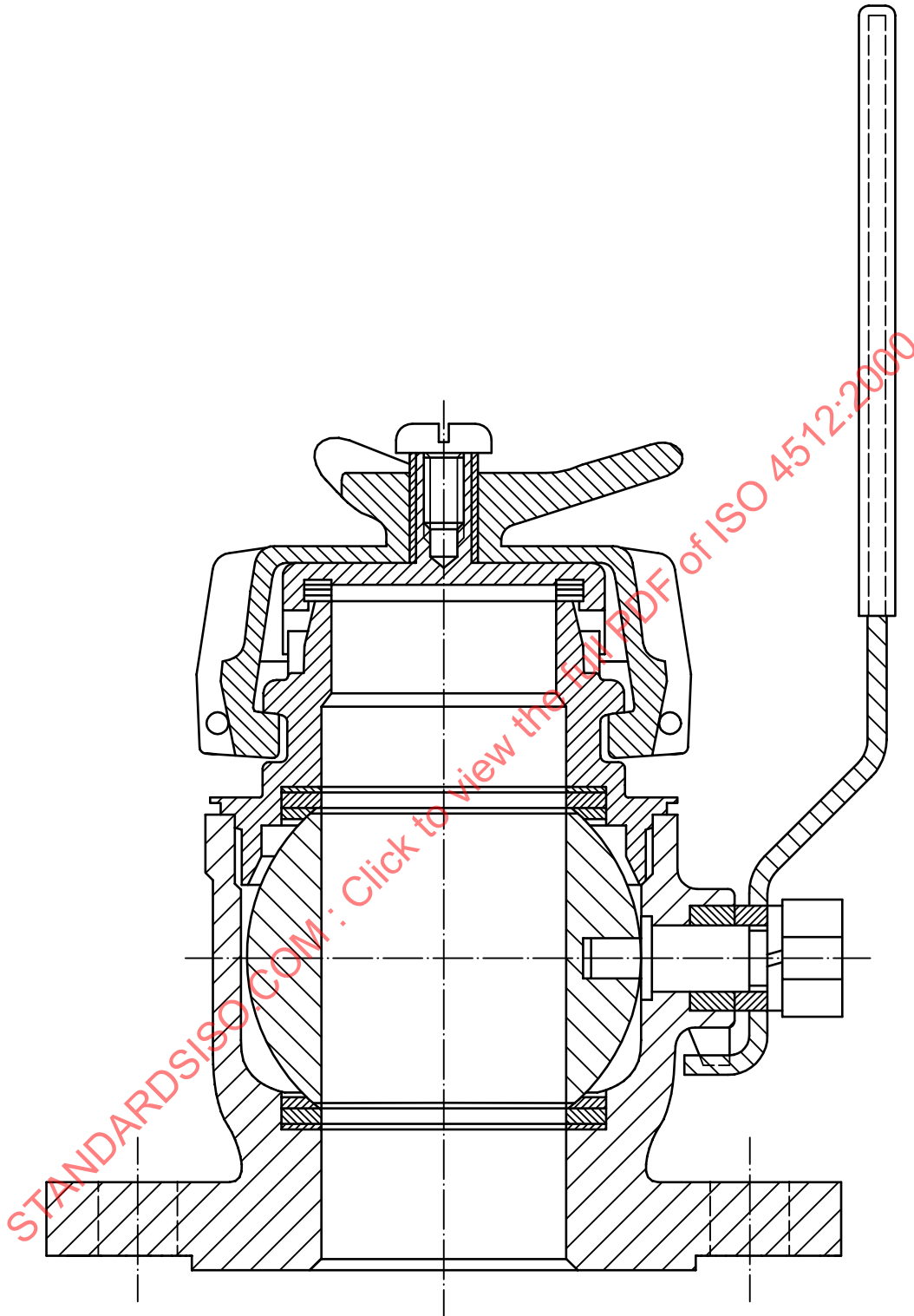
Figure 6 — Example of a typical vapour-lock valve
