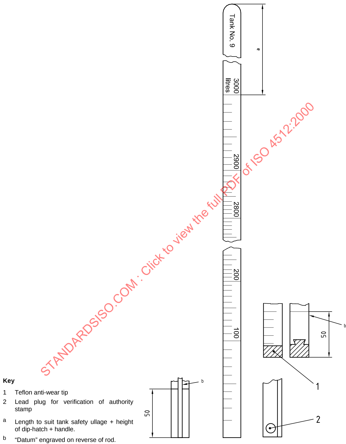
Figure 7 — Typical volumetric dip-rod
