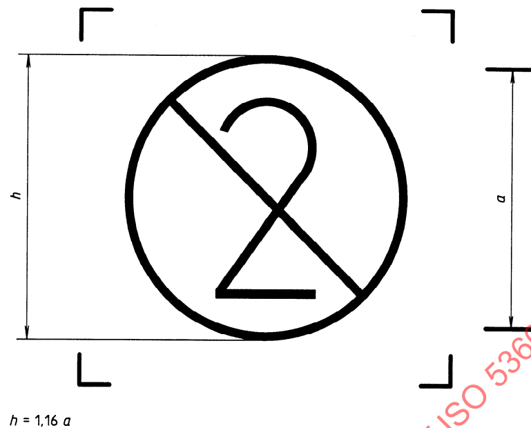
Figure 2 — ISO symbol 7000/1051 "Do not re-use"
