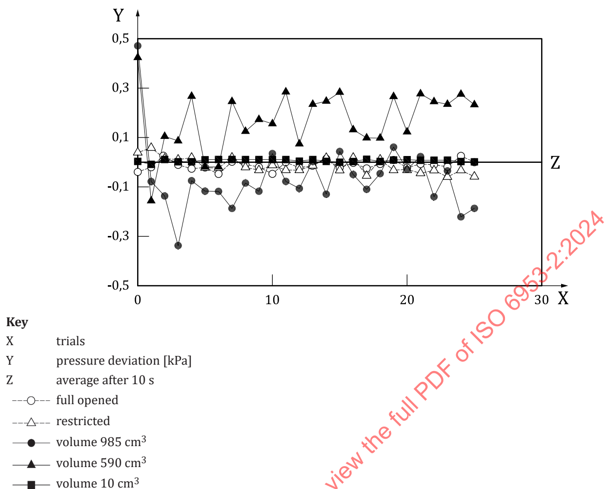
Figure A.6 — Pressure deviations after 10 s — PB1-REG
