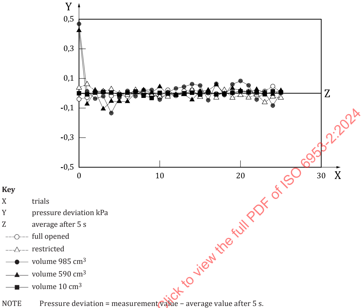
Figure A.4 — Pressure deviations after 5 s — PB1-REG
