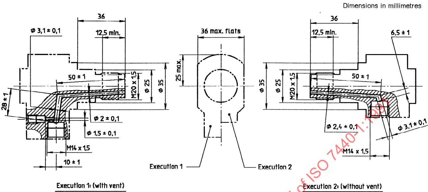
Figure 3 — Holder body
