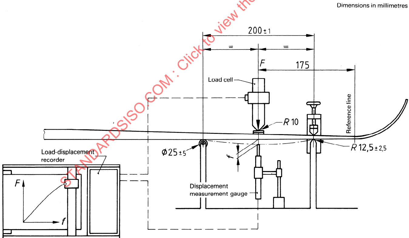
Figure 1 — Test apparatus
