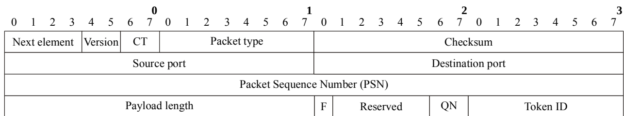
Figure 3 – Base header in ECTP-5
