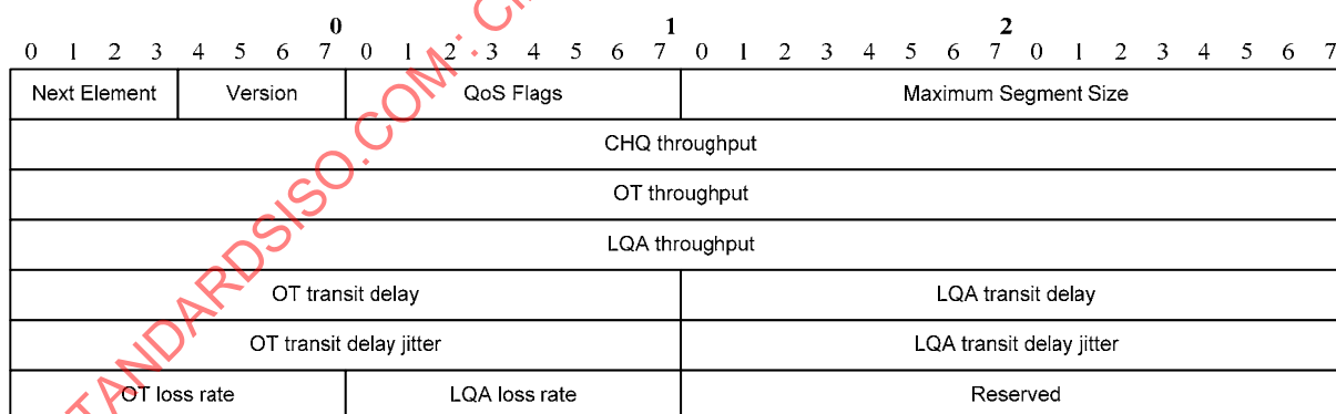
Figure 4 – QoS extension element
