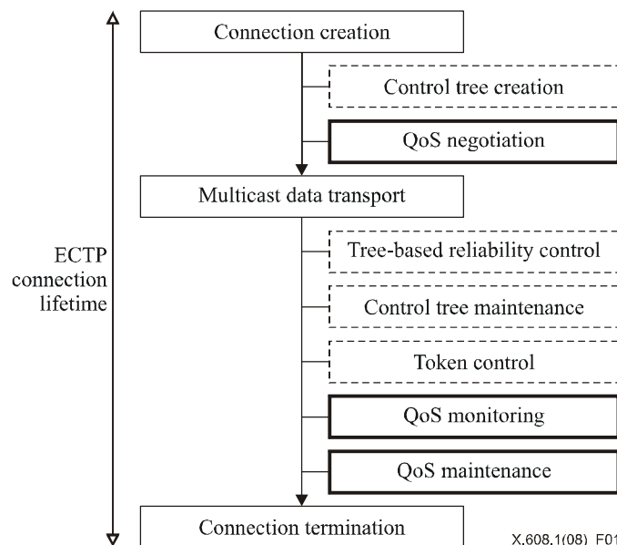
Figure 1 – QoS management in the n-plex connection
