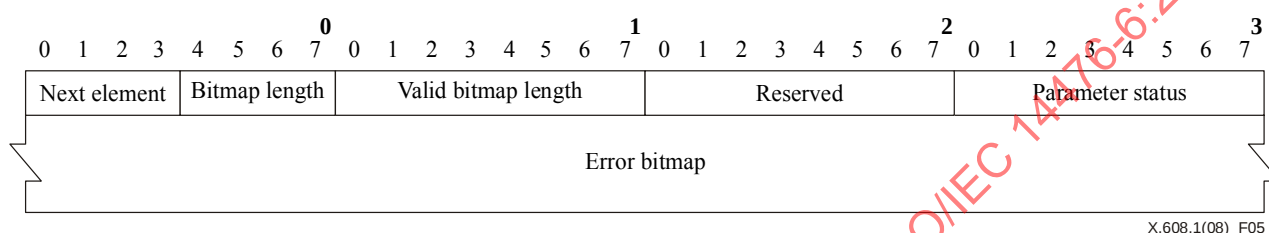
Figure 5 – Error bitmap element
