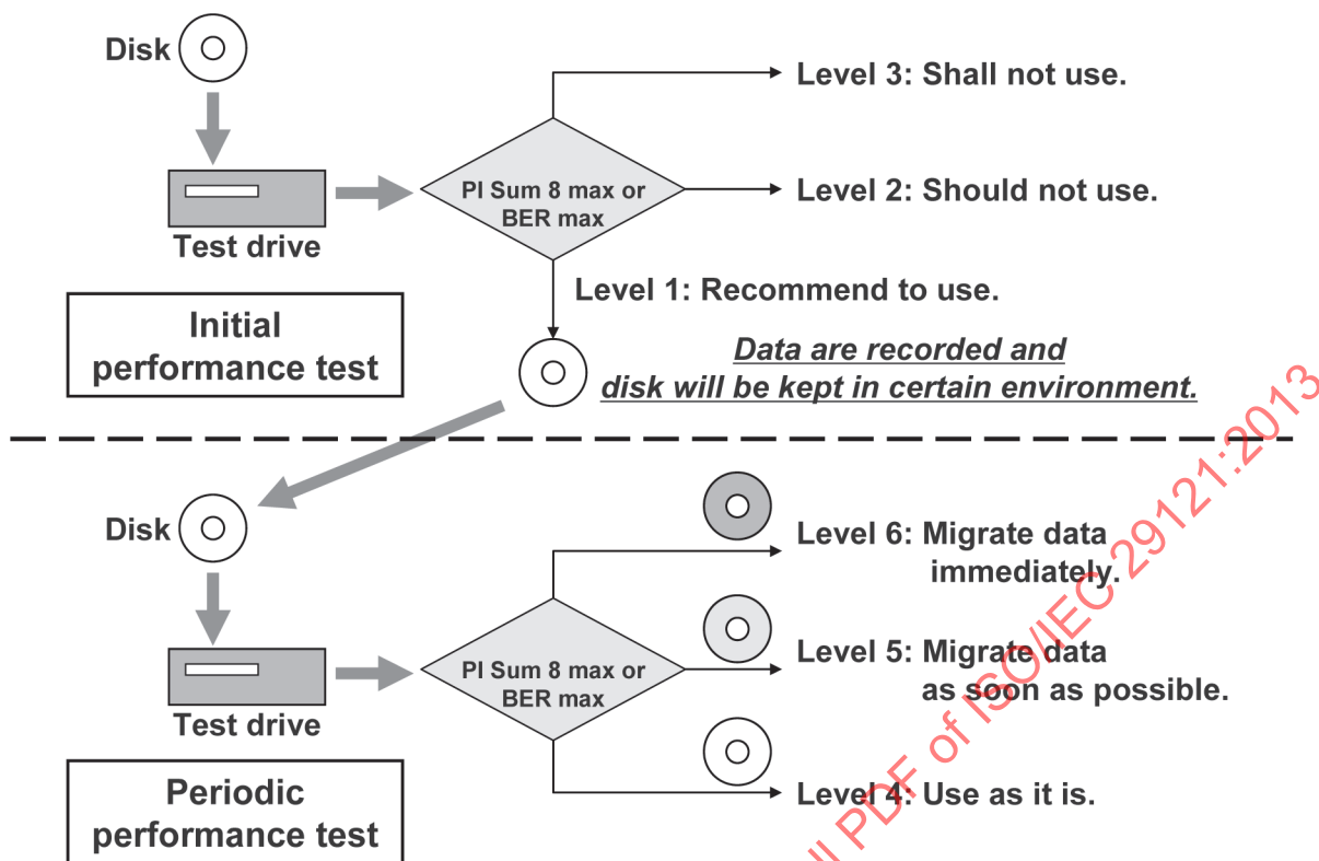
Figure 1 — Data migration flow for DVD-R, DVD-RW, DVD-RAM, +R, and +RW disks
