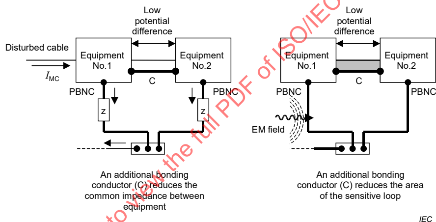
Figure 12 – Example of low common impedance and small loop
