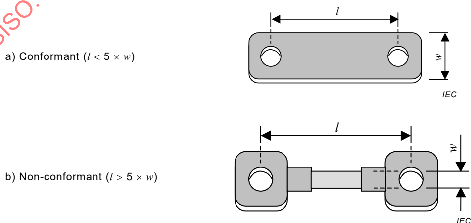
Figure 5 – Example of bonding straps
