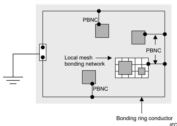
Figure 16 b – MESH-IBN via a ring protective bonding network
