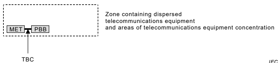
Figure 7 – Illustrative example of a smaller building
