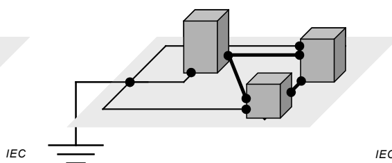
Figure 10 b – Supplementary telecommunications bonding network
