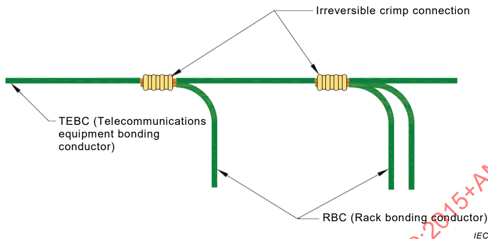
Figure 15 – Example TEBC to rack bonding conductor connection
