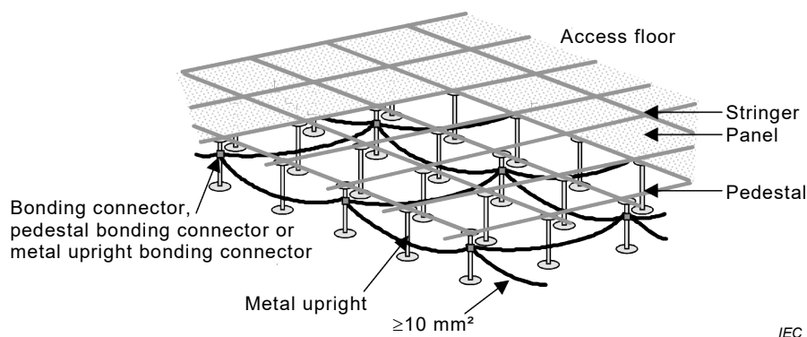
Figure 19 – Example of access floor
