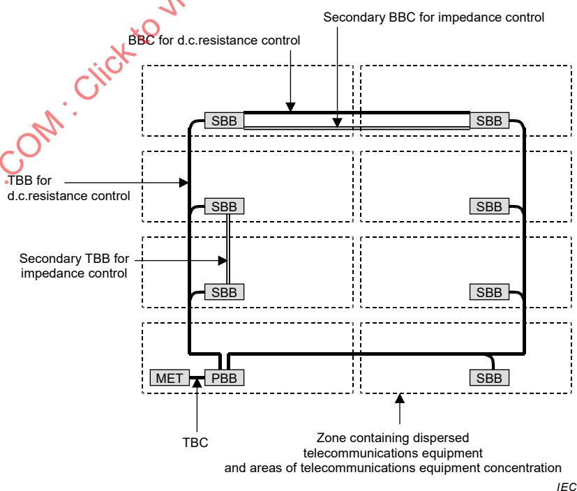
Figure 6 – Illustrative example of a large building
