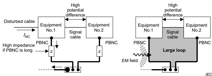
Figure 11 – Example of high common impedance and large loop
