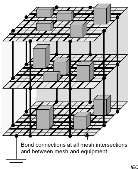
Figure 18 – A MESH-BN with equipment cabinets, frames, racks and CBN bonded together
