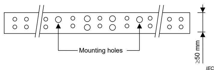
Figure 9 – Schematic of SBB
