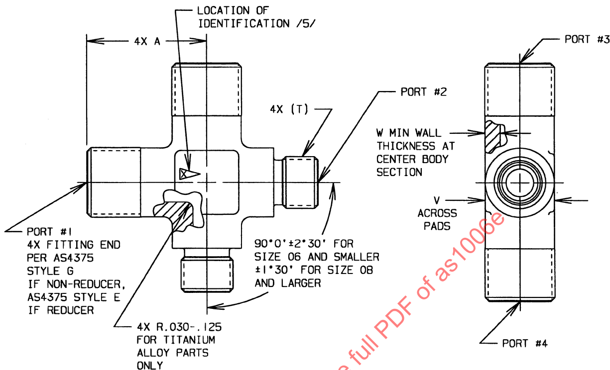
FIGURE 1 - FITTING, CROSS
