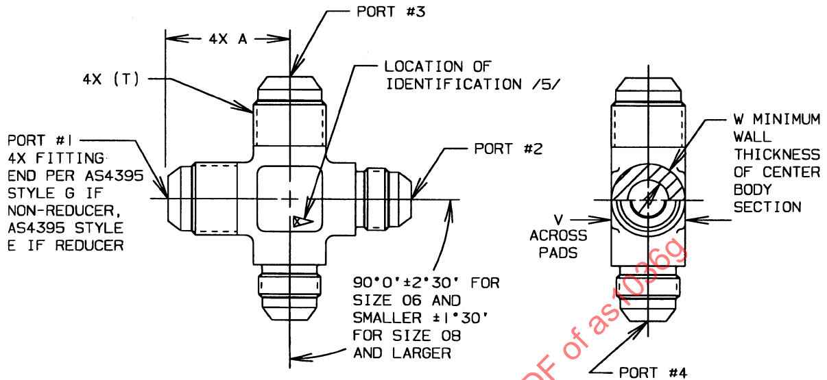
FIGURE 1 - CROSS, FLARED
