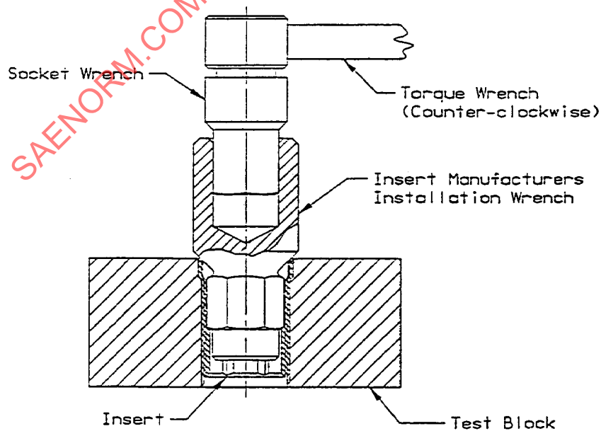
FIGURE 2 - Rotational Resistance Test Fixture
