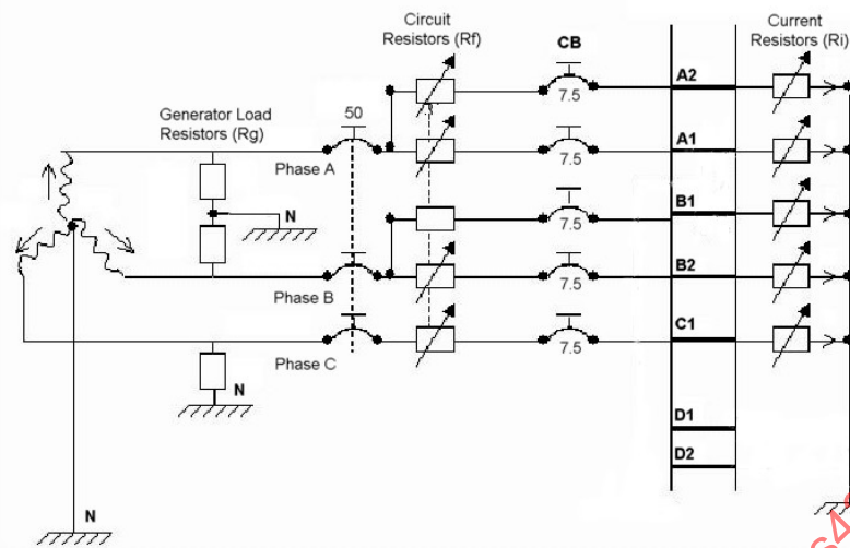
FIGURE 17 - ELECTRICAL CONNECTION
