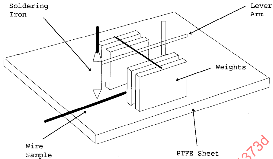
FIGURE 1 - THERMAL/MECHANICAL RESISTANCE TEST SETUP
