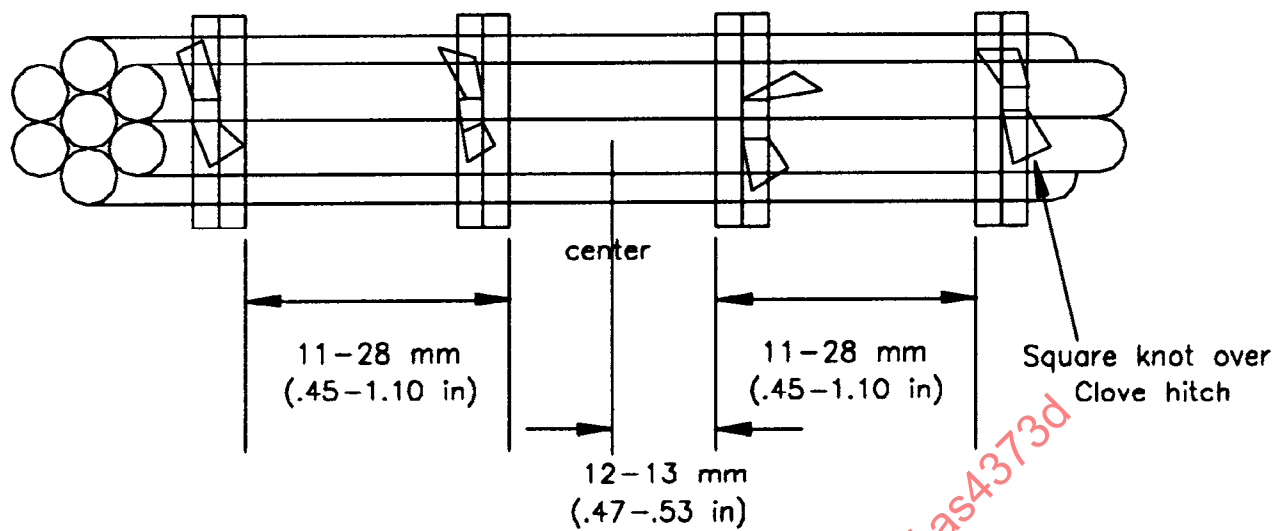
FIGURE 11 - BUNDLE TYING
