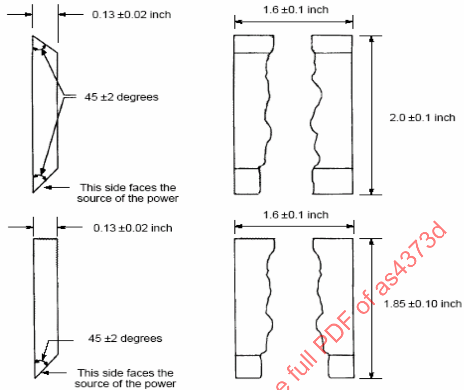
FIGURE 8 - BLADE
