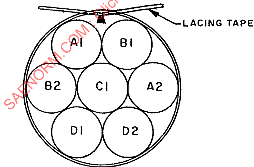
FIGURE10 - BUNDLE CONFIGURATION
