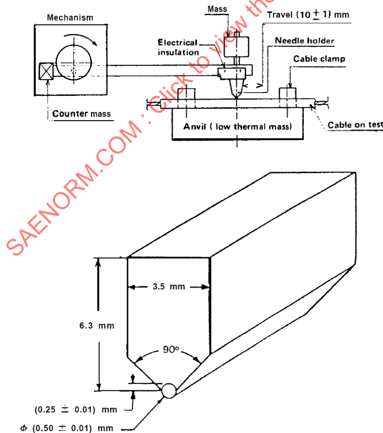
FIGURE 6 - ABRASION DURABILITY TEST FIXTURE AND NEEDLE
