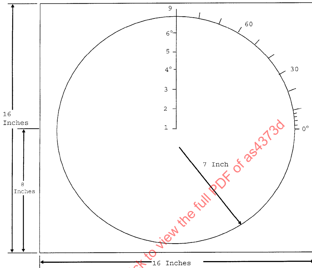
FIGURE 21 - STIFFNESS AND SPRINGBACK TEST FIXTURE BASE PLATE
