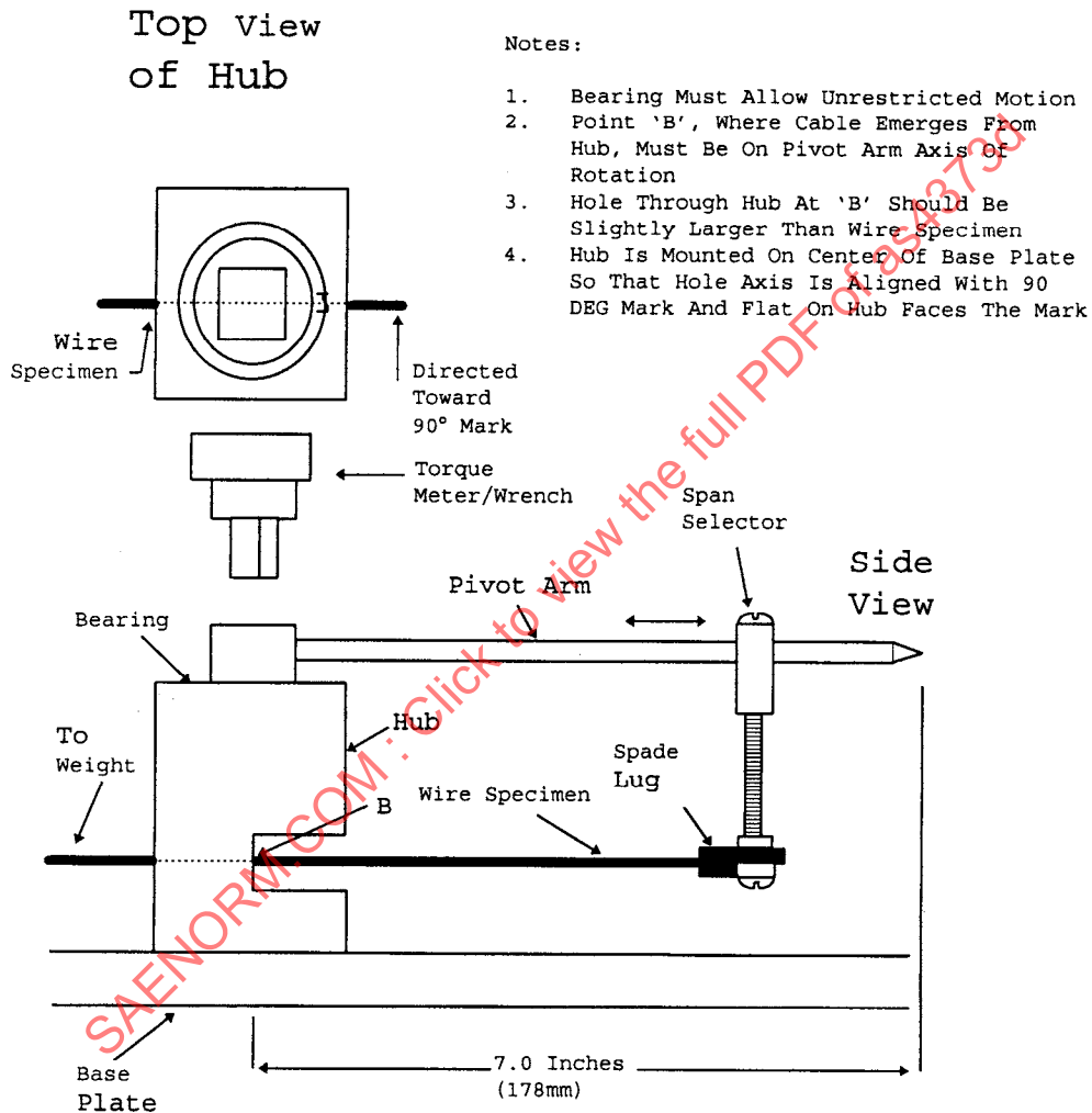
FIGURE 20 - TEST FIXTURE FOR STIFFNESS AND SPRINGBACK TEST
