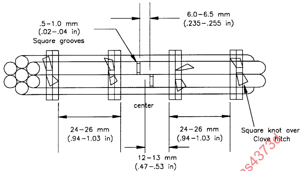
FIGURE 16 - BUNDLE TYING
