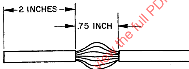
FIGURE 7 - TYPICAL 7-STRAND CONDUCTOR AFTER BIRDCAGING (NO STRANDS BLOCKED)
