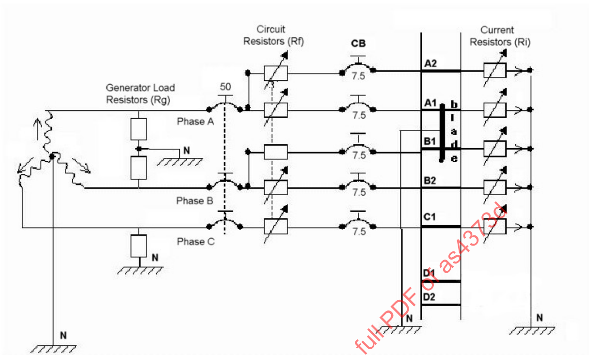
FIGURE 13 - ELECTRICAL CONNECTION
