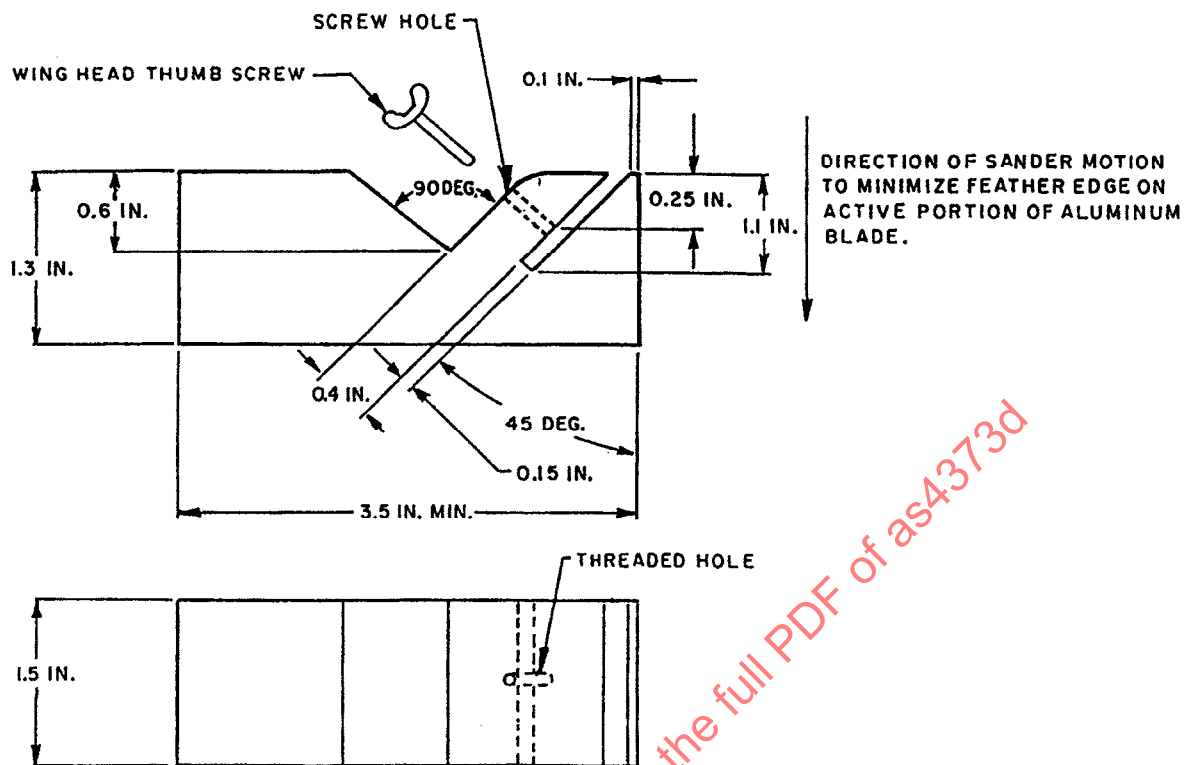
FIGURE 9 - ALUMINUM BLADE SHARPENING FIXTURE
