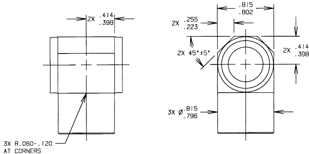
FIGURE 2 - ALTERNATE CONFIGURATION OF CENTER BODY SECTION /7/ /13/
