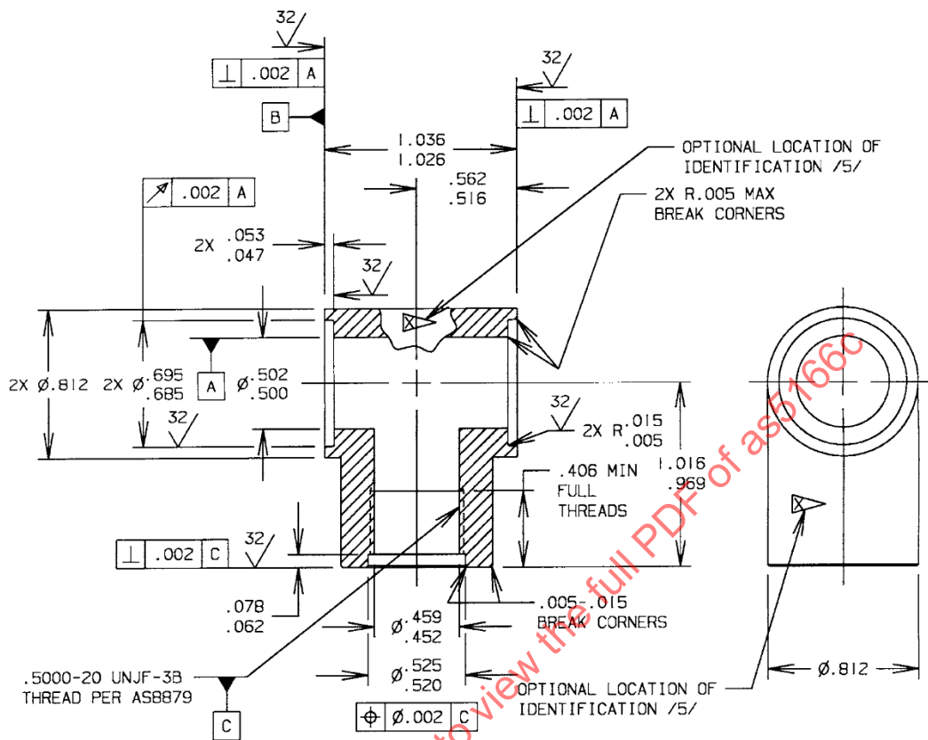
FIGURE 1 - FITTING, TEE /13/
