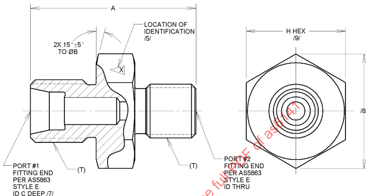
FIGURE 1 – FITTING, UNION AND REDUCER
