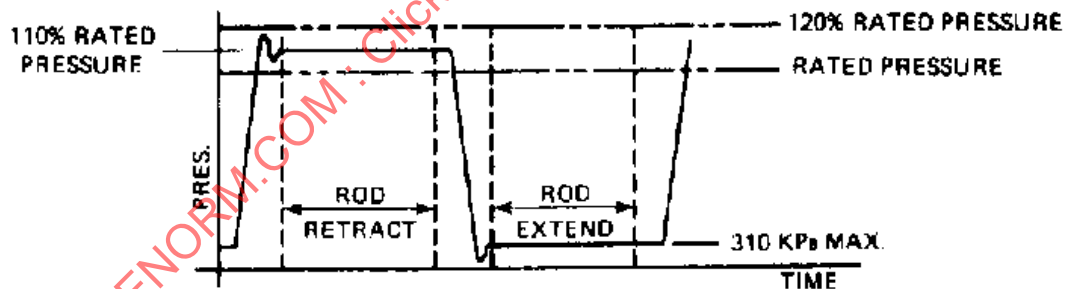
Figure 3 - Typical pressure-stroke cycle
