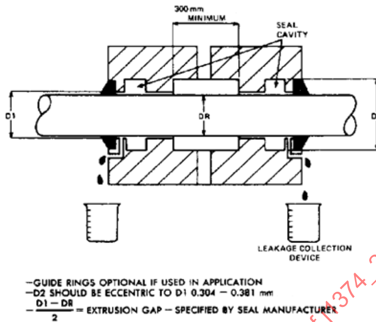
Figure 2 - Rod seal test chamber (typical)
