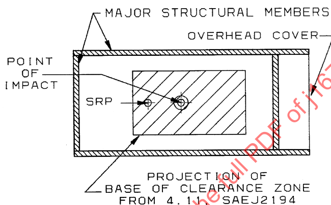
FIGURE 2—DROP TEST POINT OF IMPACT
