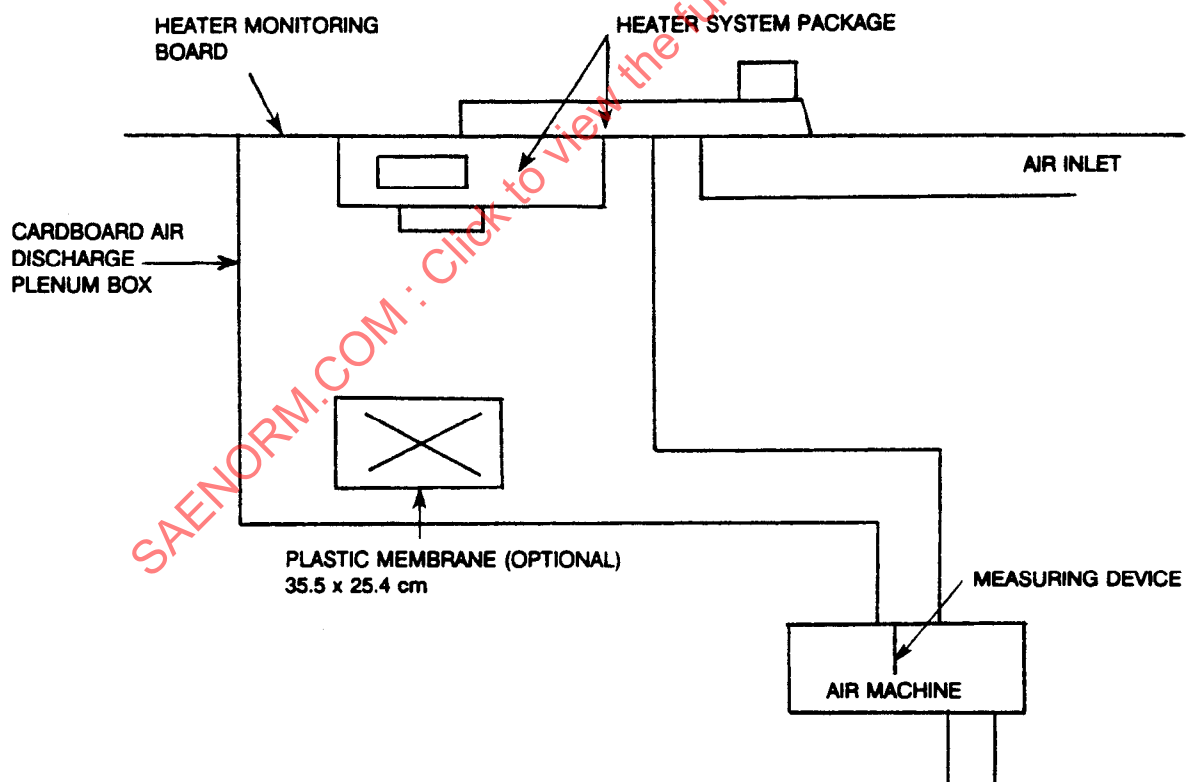
FIGURE 1—BENCH TEST SET-UP
