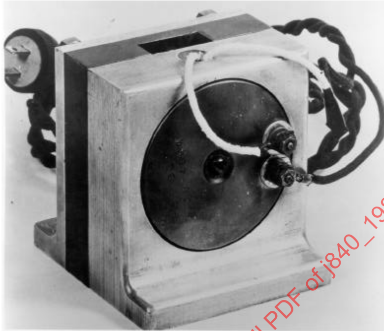
FIGURE 10—DISC SHEAR FIXTURE
