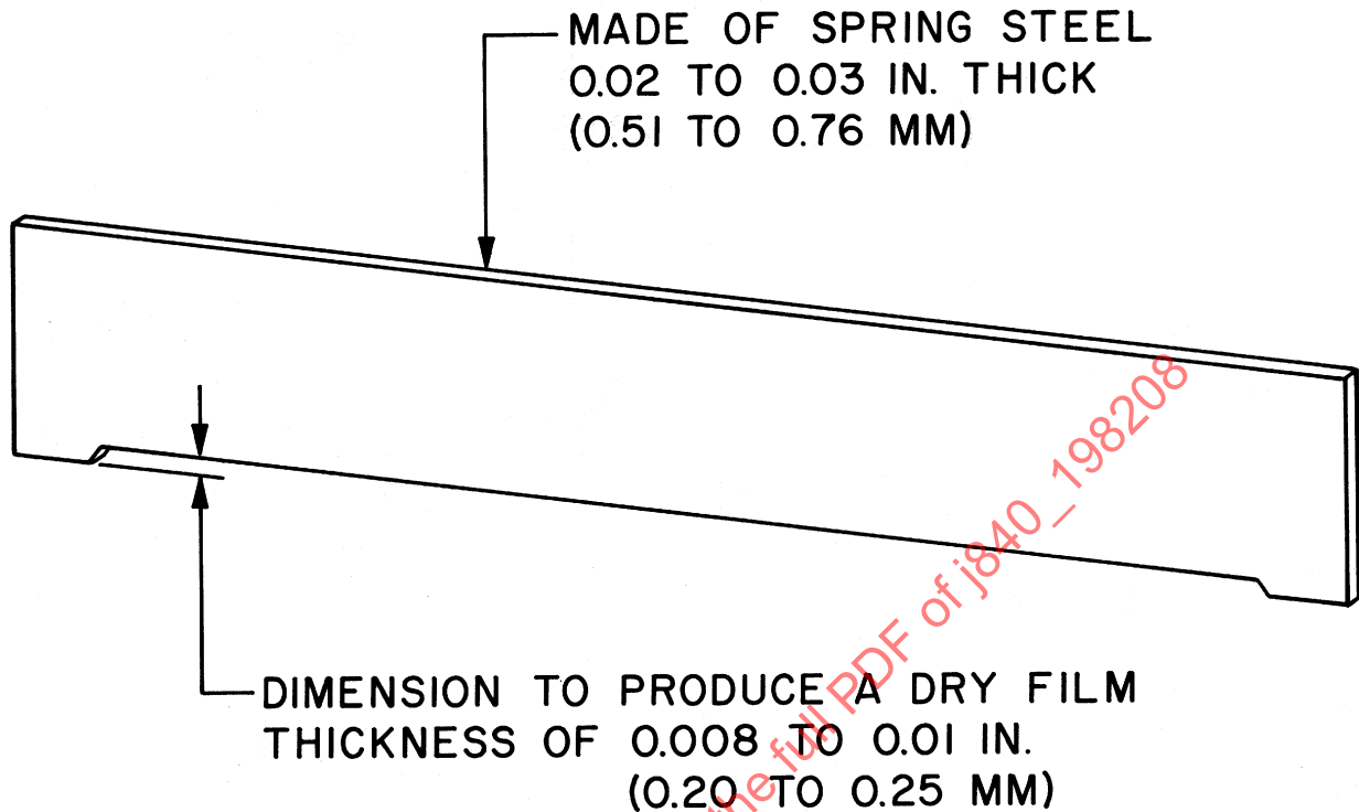
FIGURE 7—DOCTOR BLADE
