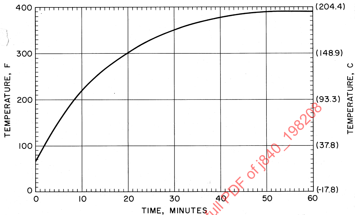
FIGURE 9—RATE OF HEATING CHANGE
