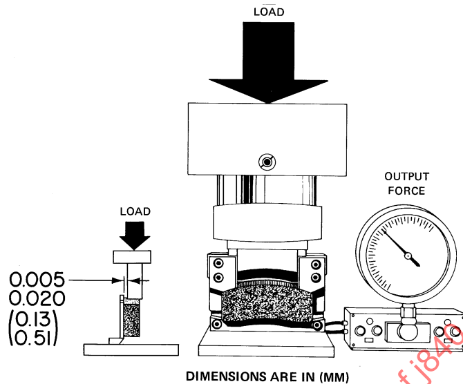
FIGURE 2—DISC BRAKE SHEAR TEST FIXTURE
