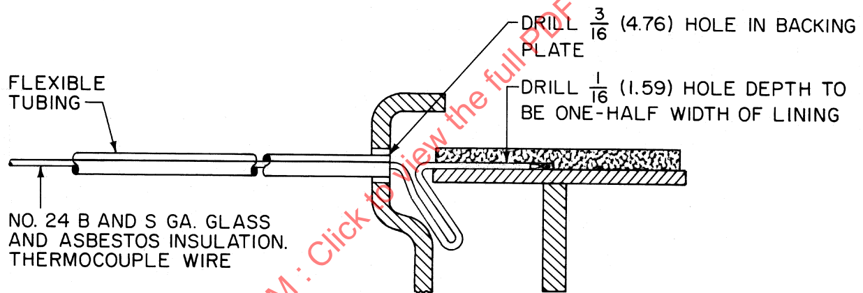
FIGURE 4A—DRAWING OF THERMOCOUPLE LOCATION—DRUM BRAKE
