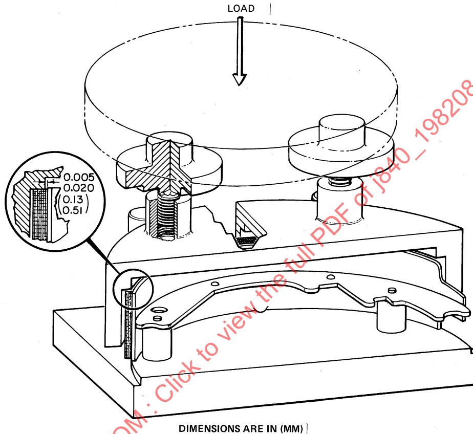
FIGURE 1—BOND PLANE SHEAR TEST—DRUM BRAKE
